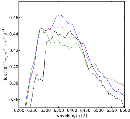
Figure 11. Synthetic spectrum at -3 d produced using the W7e0.7 density profile to constrain an upper limit on carbon. The blue line is the model with 0 per cent of C, the red dashed line with the 2 per cent C and the green line with 10 per cent C at the photosphere. The black line is the observed spectra.
