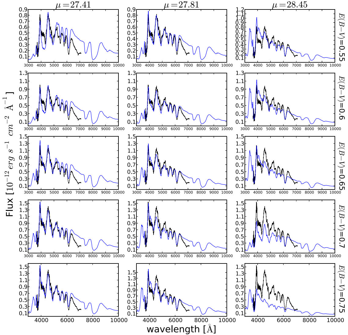
Figure 3. One-zone models of SN 1986G at B -band maximum, using a variety of distance modulus and extinction values. The observed spectra are in black and the modelled in blue.
