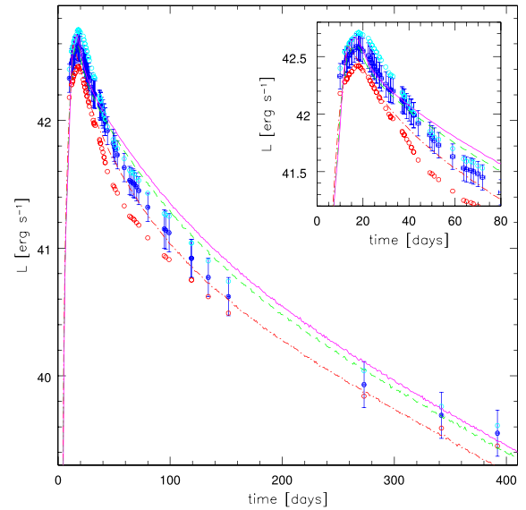
Figure 14. The observed (blue dots) bolometric LC with the upper (cyan markers) and lower (red markers) limits. As well as the modelled LC using the derived abundance distribution from the W7 (green), Sub-Ch (red) and W7e0.7 (purple) density profiles.
