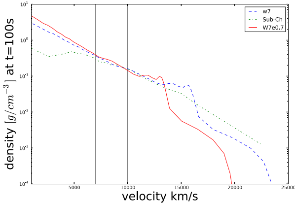
Figure 8. The W7, Sub-Ch and W7e0.7 density profiles as a function of velocity at t = 100 s after explosion. The vertical grey lines show the range in values v_{ph} can take, for the -3 d to +2 d models.
