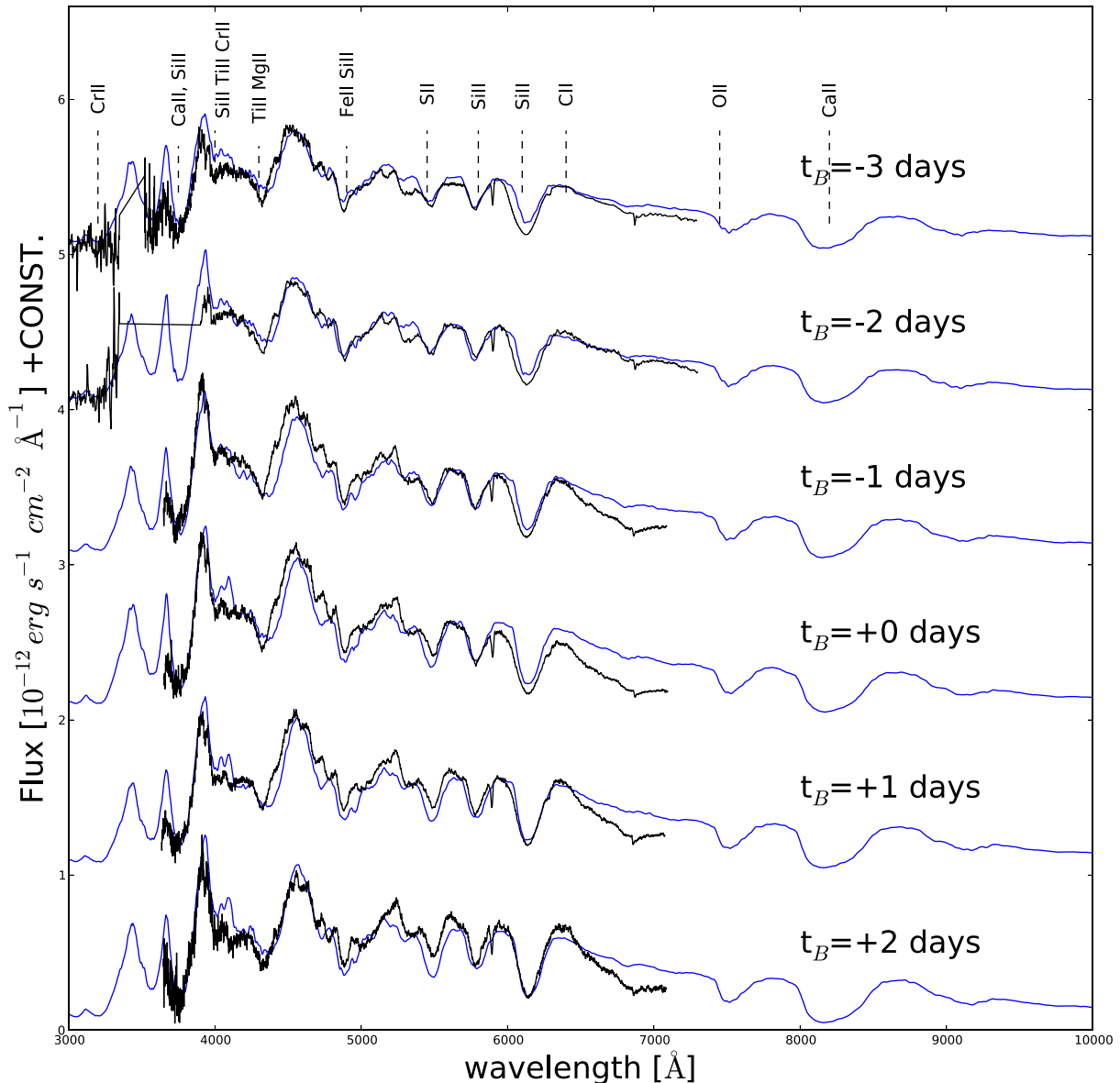
Figure 10. The photospheric phase models of SN 1986G, calculated using the W7e0.7 density profile. The blue line are the models and the black line the observed spectra. The spectra have been corrected for extinction.
