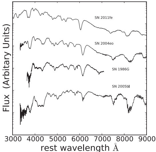
Figure 2. The spectra of four SNe Ia at B -band maximum. The SNe correspond to the 4 SNe in Fig. 1.
