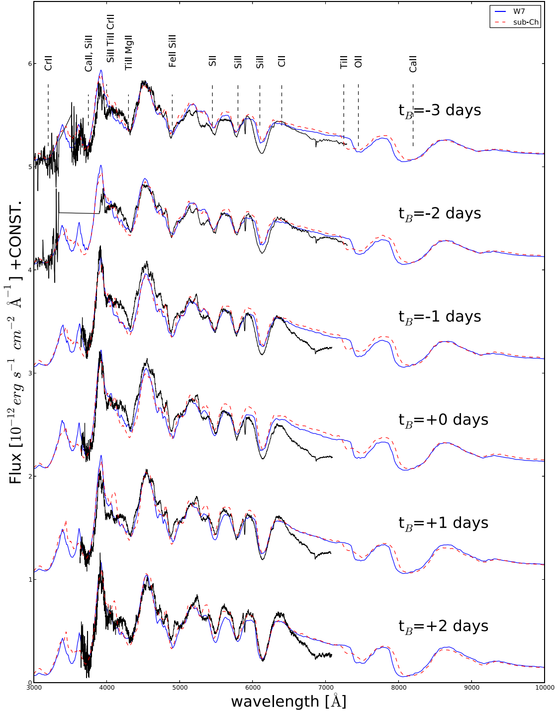
Figure 4. The photospheric phase models of SN 1986G, where the spectra have been shifted in flux by a constant for clarity. Models for both the W7 (blue solid) and Sub-Ch (red dashed) density profiles are shown. The spectra have been corrected for extinction.
