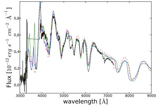
Figure 9. One-zone models at -3 d relative to B -band maximum. The synthetic spectra were produced using the W7 (blue), W7e0.7 (green) and Sub-Ch (red dashed) density profiles. The spectra have been corrected for extinction.
