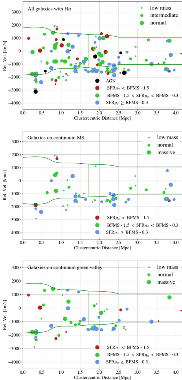
Figure 9. Top: the distribution of the 158 galaxies with H \alpha in relative velocity–clustercentric distance space. The galaxies are colour coded according to their position within \log(\text{SFR}) versus \log(M_{\text{stellar}}) space, while the AGN candidates are plotted in black. The points are further plotted in three sizes, corresponding to the ‘low-’, ‘intermediate-’, and ‘normal-mass’ bins defined earlier. The caustic edges and r_{200} = 1.73 Mpc are also displayed, to separate the core, outskirts, and infalling regions. Passive galaxies (those without H \alpha detection) are omitted in the plot, but are also present throughout all regions of the cluster (see Fig. 10). Middle: the distribution of the 61 galaxies originally on the continuum main sequence. The colours are the same as above; the blue galaxies have maintained their SFRs, while the green points have been suppressed. Bottom: same as the above, but for the distribution of 48 galaxies within the continuum green valley. The blue points have experienced a recent increase in star formation.
