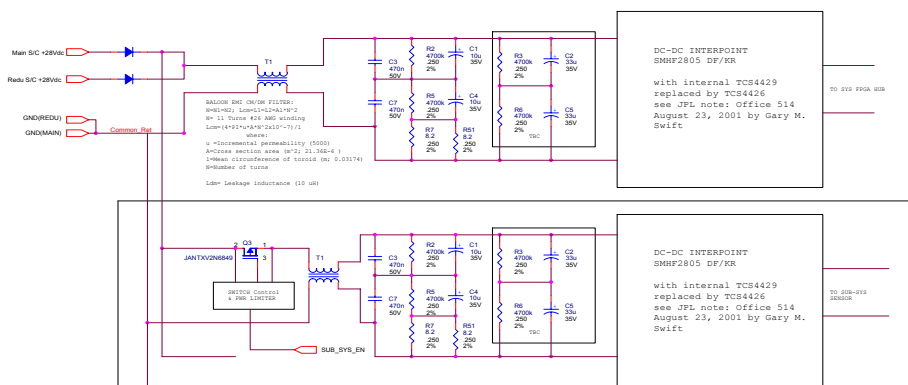
Figure 4.6. NSWDC power distribution block diagram.
