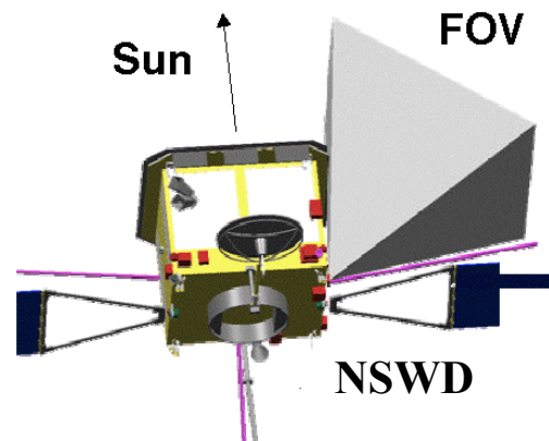
Figure 3.6. Potential instrument location on Solar Orbiter and field of view of NSWDF.
