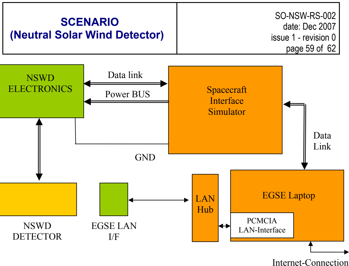
Figure 6.1. EGSE functional block diagram
