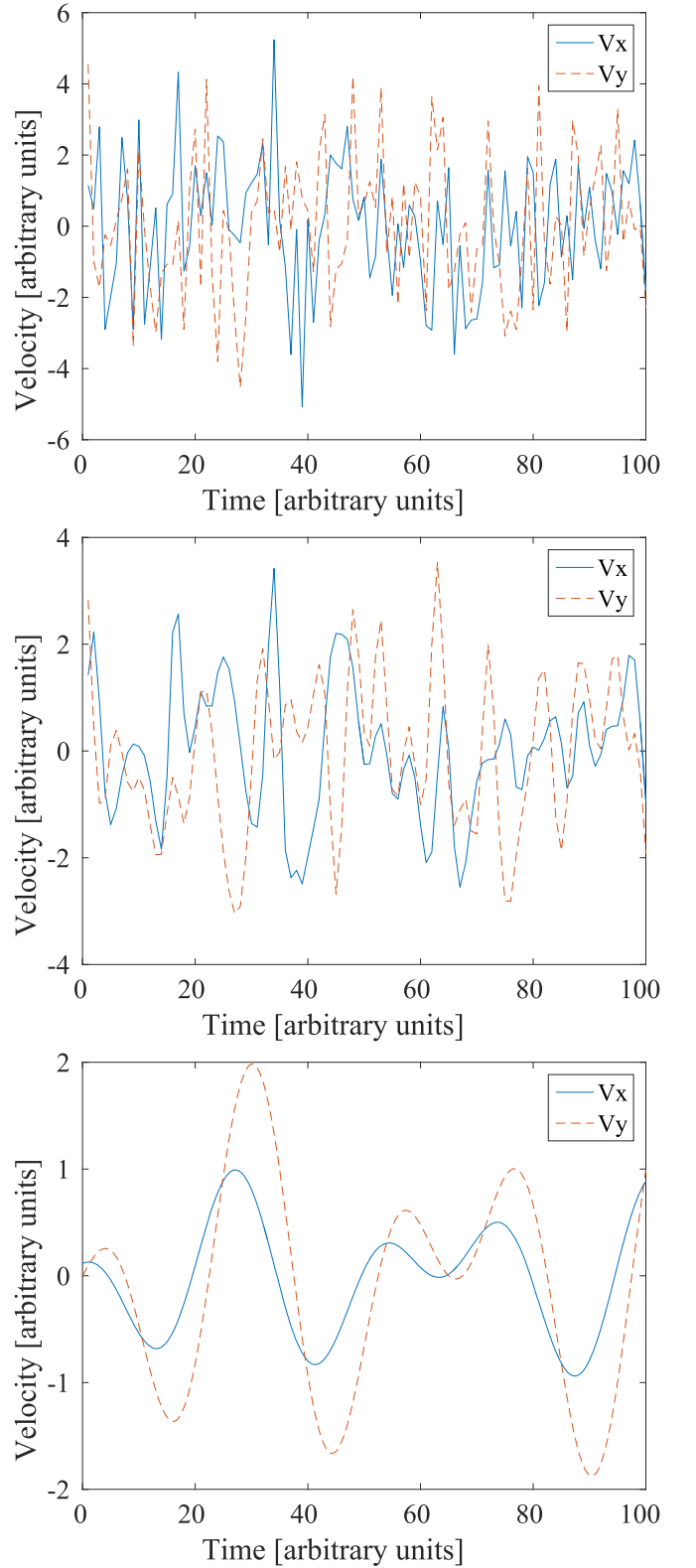
Figure 8. Top panel: simulated random velocity signal with normal distribution. Middle panel: same velocity signal filtered using the EMD. Bottom panel: simulated velocity signal made with two superimposed pulses in the x and y direction respectively. The two pulses are exactly the same, but slightly shifted and with different amplitudes.
