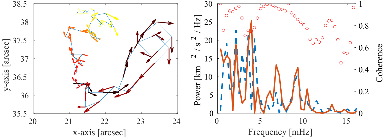
Figure 4. Left panel: trajectory in time \dot{s}(t) of the magnetic element marked with a red star in Figure 2, with the velocity vector \dot{s}(t) superimposed. The colors encode the temporal evolution, from dark red to light yellow. Right panel: periodogram of the two components of \dot{s}(t) ( v_x : red line, v_y : dashed blue line). In the same plot, we also show with the coherence spectrum between these two components, smoothed with an averaging window 3 points wide (red circles).
