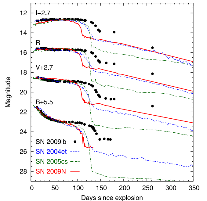
Figure 3. Comparison of the BVRI light curves of SNe II-P. The light curves were vertically shifted so their peak magnitudes match those of SN 2009ib in each band. The explosion epochs of the comparison SNe are very well constrained (Table 1). The diversity of the shapes is reflected mostly in the length of the plateau and the drop to the tail. SN 2009N (red) has the same brightness as SN 2009ib (black circles), however its plateau is shorter. SNe 2005cs (green) and 2004et (blue) have about the same plateau length, but their absolute brightness differ by more than 2 mag and the drop in the end of the plateau of SN 2005cs is greater.
