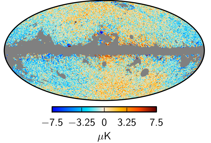
Fig. A.4. Difference between the Commander CMB solutions derived using (1) only Planck data and (2) Planck +WMAP+408 MHz, both smoothed to a common resolution of 1^\circ FWHM. The grey region indicates the common mask.
