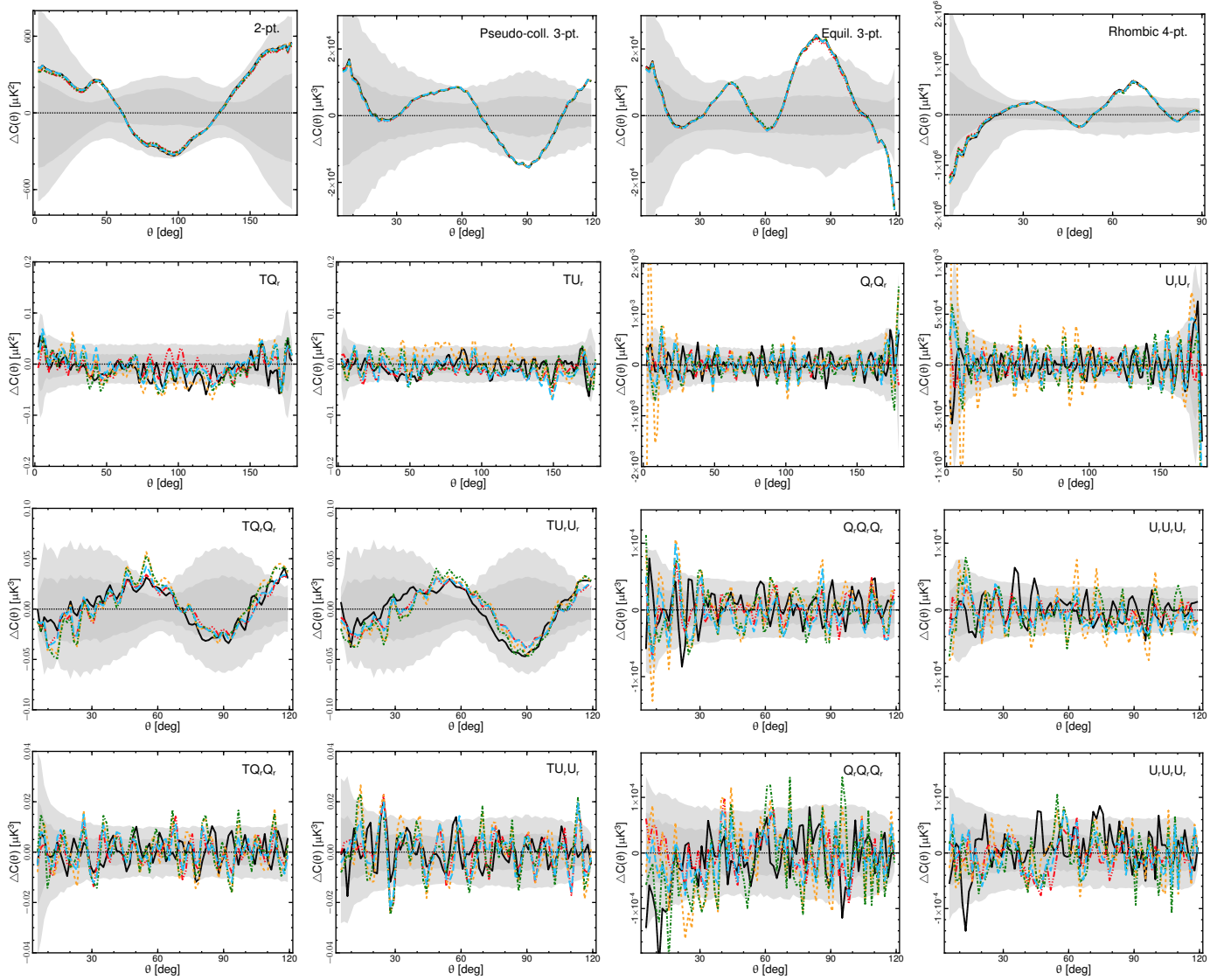
Fig. E.4. Difference between the N -point functions for the high-pass filtered N_{\text{side}} = 64 FFP8 CMB estimates and the corresponding means estimated from 1000 MC simulations. The Stokes parameters Q_r and U_r were locally rotated so that the correlation functions are independent of coordinate frame. The first row shows results for the temperature map, from left to right , results for the 2-point, pseudo-collapsed 3-point, equilateral 3-point and connected rhombic 4-point functions. We note that the lines lie on top of each other. The second row shows results for the 2-point function, from left to right , TQ_r , TU_r , Q_rQ_r , and U_rU_r . The third row shows results for the pseudo-collapsed 3-point function, from left to right , TQ_rQ_r , TU_rU_r , Q_rQ_rQ_r , and U_rU_rU_r , and the fourth row shows results for the equilateral 3-point function, from left to right , TQ_rQ_r , TU_rU_r , Q_rQ_rQ_r , and U_rU_rU_r . The black solid, red triple-dot-dashed, orange dashed, green dot-dashed, and blue long dashed lines correspond to the true, Commander, NILC, SEVEM, and SMICA maps, respectively. The true CMB map was analysed with added noise corresponding to the SMICA component separation method. The shaded dark and light grey regions indicate the 68% and 95% confidence regions, respectively, estimated using SMICA simulations. See Sect. 7.2 for the definition of the separation angle \theta .
