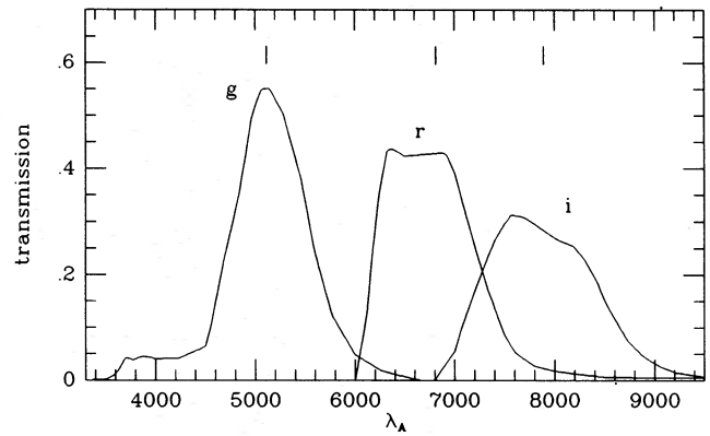
Figure 1. Response curves for the photometric system used in this work. The absolute transparency of ESO-Gunn filter + CCD #8 + EFOSC camera is plotted. Effective wavelengths are marked on the top.
