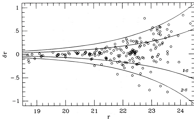
Figure 7. Distribution of the magnitude differences of the same objects measured in two different r frames of comparable exposure times (i.e. 20 and 25 min). Solid lines encompass 1\sigma and 2\sigma envelopes. Mean standard deviation is 0.17 mag at r = 22 .
