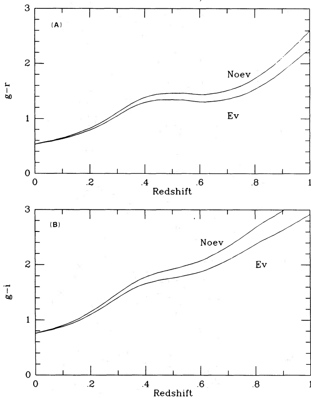
Figure 18. Expected colours ( g-r ) (panel A) and ( g-i ) (panel B) for elliptical galaxies, in the case of passive ( Noev ) and active ( Ev ) photometric evolution, as discussed in the text. Synthetic colours are based on the models for evolutionary population synthesis by Buzzoni (1989), and assume an (H_0, q_0) = (50, 0) cosmology.
