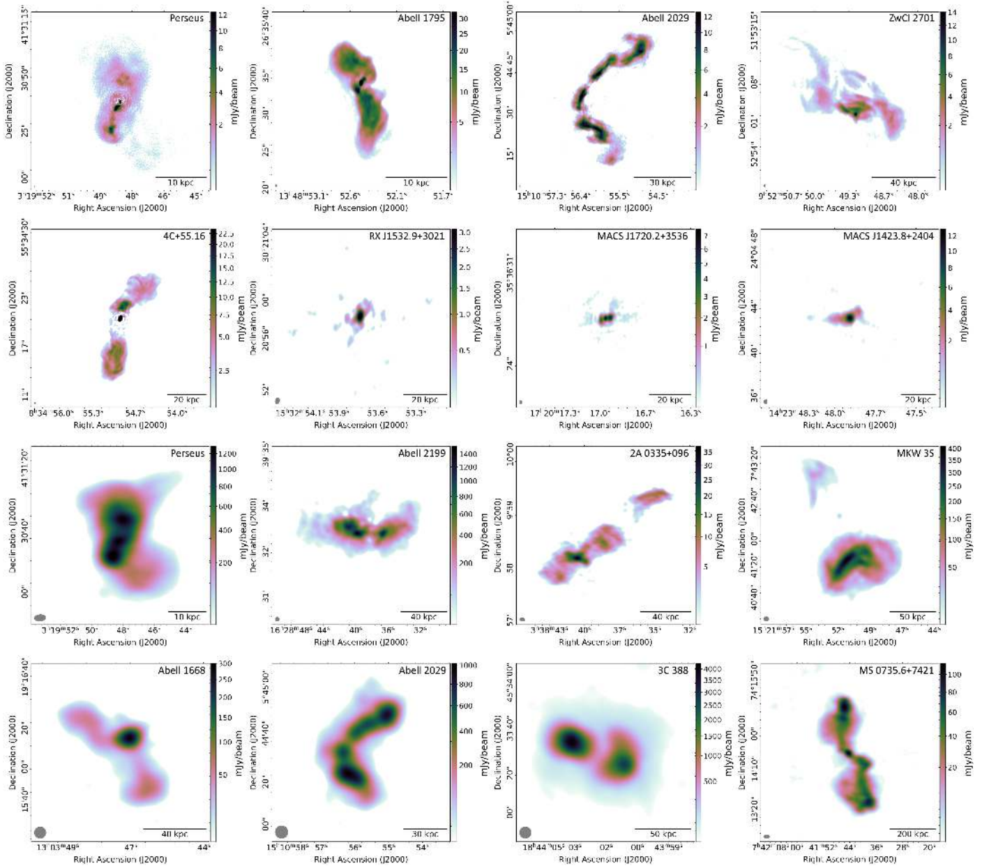
Fig. 1. LOFAR images of all galaxy clusters our the sample. The top 8 panels show the high-resolution maps produced by including LOFAR's international stations and the bottom 8 panels show the low-resolution maps produced using only the Dutch part of the array. Note that Perseus and Abell 2029 are presented in both sections. The central dominant compact component in the Perseus cluster was peeled from the data for the low-resolution map for calibration purposes. The color maps range from three times the rms noise level to the peak brightness, except in the cases of Perseus, Abell 1795 and 4C+55.16, for which the peak brightness of the lobes was used due to the otherwise dominant central compact component. The scale bar in the bottom right corner of each panel measures the listed length at the redshift of the respective clusters. The beam is indicated in grey in the bottom left corner of each panel.
