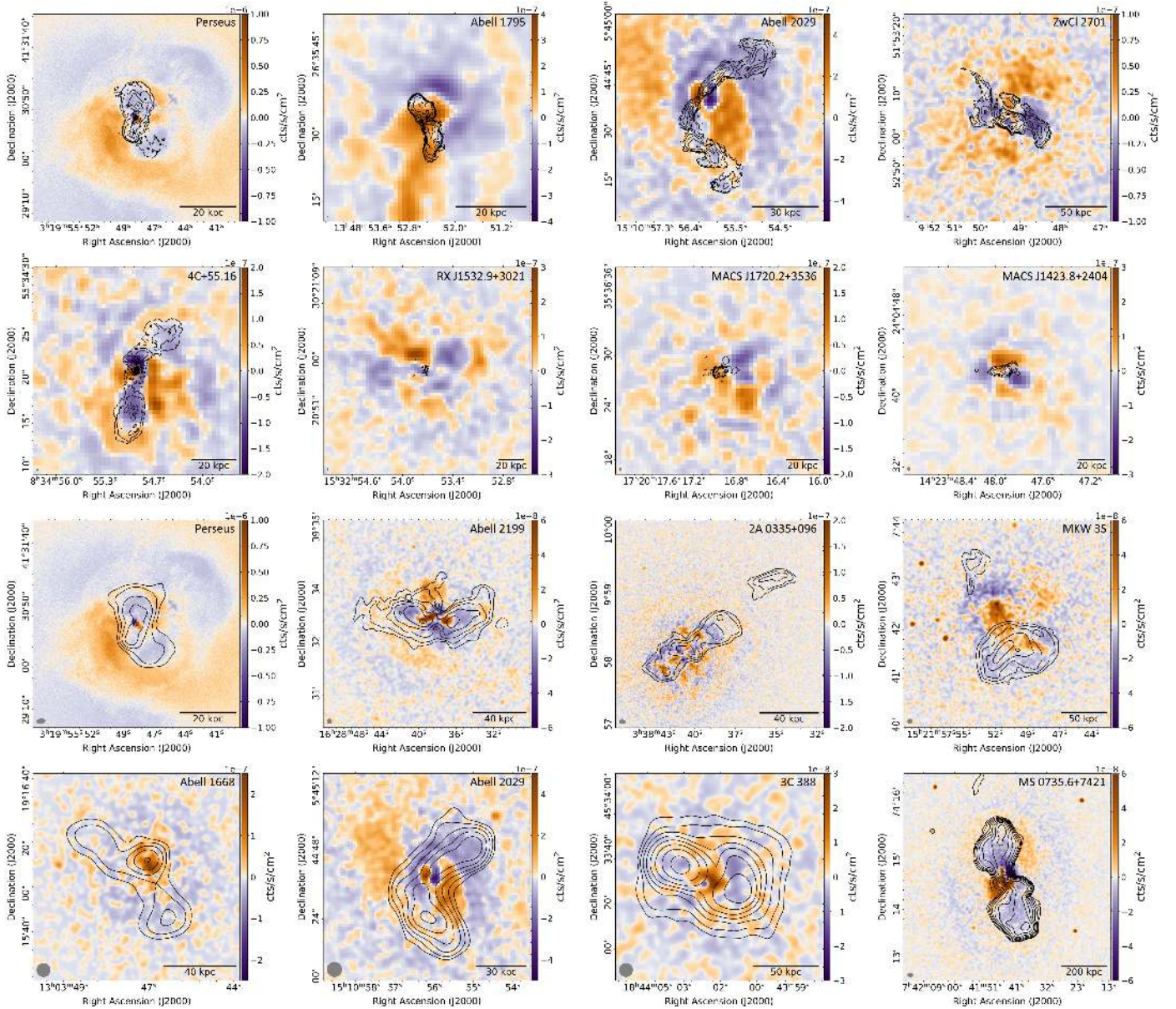
Fig. 2. Residuals from the Chandra X-ray images after subtracting a smooth model of the ICM surface brightness. The top 8 panels show the X-ray residual maps corresponding to the high-resolution sample and the bottom 8 panels show the X-ray residual maps corresponding to the low-resolution sample. Note that Perseus and Abell 2029 are presented in both sections. The orange and purple colors indicate regions with surface brightness excess and deficiency, respectively. The black contours indicate the radio emission, and are drawn in increments of factors of 2, starting at 5 times the rms noise level. The scale bar in the bottom right corner of each panel measures the listed length at the redshift of the respective clusters. The beam is indicated in grey in the bottom left corner of each panel.
