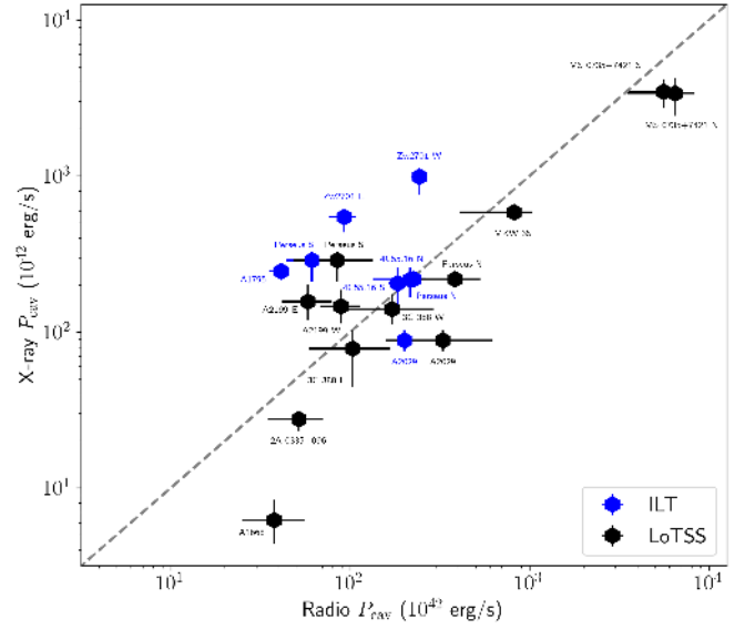
Fig. 5. The hybrid X-ray–radio cavity power measurements versus the purely X-ray-based cavity power estimates. The blue data points indicate the measurements derived using high-resolution observations, while the black data points indicate the measurements derived using low-resolution observations.
