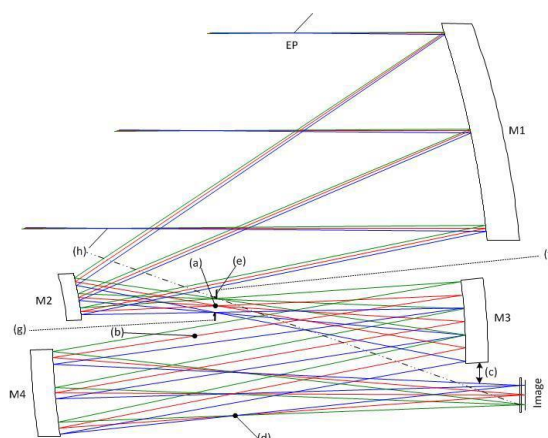
Figure 6 Ray tracing via ZEMAX code of the CaSSIS 135 optical system. The TMA configuration has an intermediate focal plane (a) and two intermediate walls (f and g) which subdivide the telescope into an upper compartment with M1 and M2 and a lower compartment with M3 and M4 separated with baffles to avoid direct light in to the detector through the field stop. The powered folding mirror M4 allows maintaining compact design and telecentric system.
