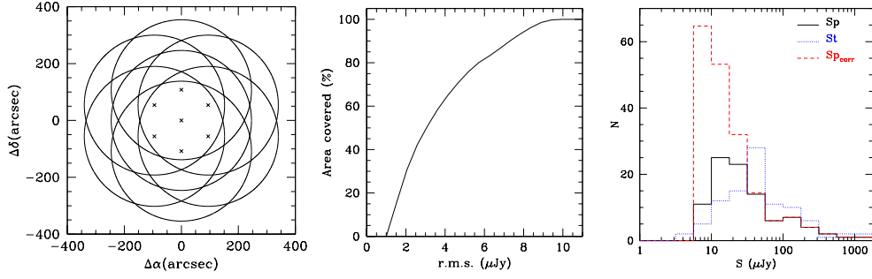
Figure 2: Left: mosaic pattern of the 7 pointing centers (crosses) at 5.5 GHz. The full circles show the primary beam of the JVL A ( \sim 10 arcmin) at this frequency. The plot clearly illustrates that the region observed is oversampled. The J2000 coordinate of the central pointing are \alpha = 12^{\text{h}}36^{\text{m}}49^{\text{s}}.4 , \delta = +62^{\circ}12'58'' . Center: visibility function of the 5.5 GHz mosaic (area vs rms sensitivity) calculated over the region used to derive the source catalog (see text). Right: observed peak (continuous black line) and total flux densities (dotted blue line) distribution of the 5.5 GHz sources. The dashed red line indicates the peak flux density histogram after correcting for the visibility function.
