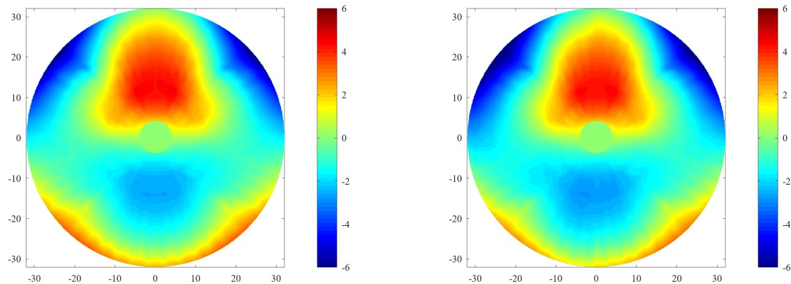
Figure 9. Maps of deflections detected at 80^\circ elevation angle. The left map refers to the case in which only gravitational load is applied; the right map refers to the case in which to the gravitational load has been added a 5^\circ\text{C} thermal load to the right half of the BUS ( x_+ side). The abscissae and ordinates are expressed in metres, while the deflections are expressed in millimetres.
