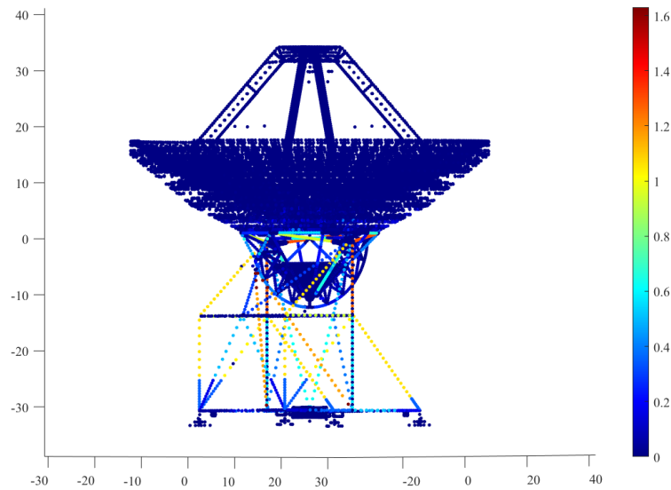
Figure 2. Map of the influence on the pointing of each element of the finite element model with elevation angle equal to 90°. The colour gradation of each point in the map represents the amount of PVR (expressed in arcsec) produced by the element it represents.
