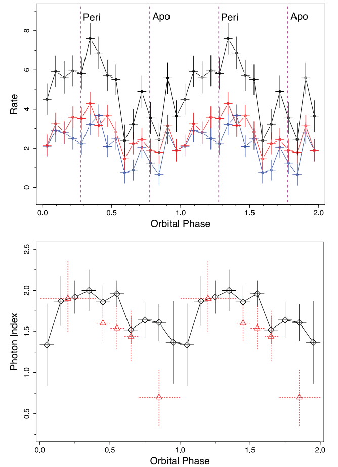
Figure 5. Upper panel: folded BAT light curve (15–110 keV range) at P_{\text{orb}} = 26.496 d. Time zero of reference MJD 43 366.275. Red, blue, and black curves are data selected in the 15–35, 35–150 and 15–150 keV ranges, respectively. Magenta dotted lines indicate the periastron and apoastron phase passages (Aragona et al. 2009). The BAT rate is in units of 10^{-5} counts \text{s}^{-1} pixel ^{-1} . Lower panel: the photon index of the power law that best fits the data in the 15–150 keV range as a function of the orbital phase. We also show for comparison the values obtained with INTEGRAL /ISGRI data (red triangles) according to Li et al. (2014). Two periods shown for clarity.
