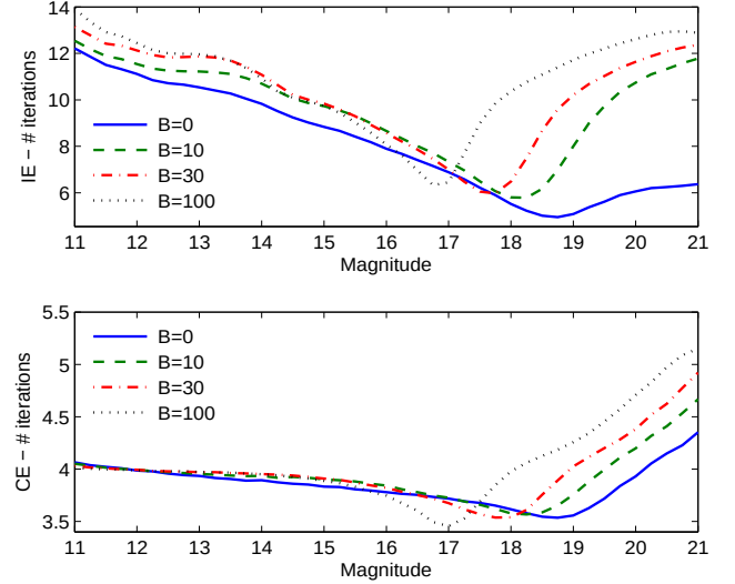
Figure 8. Mean number of iterations required for convergence by IE (top) and CE (bottom)
