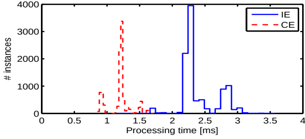
Figure 9. Histogram of processing time for IE and CE, G = 15 \text{ mag} , B = 10 \text{ photons/pixel}
