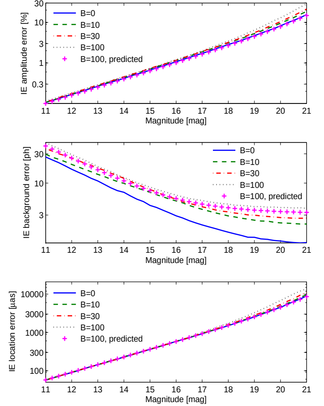
Figure 4. IE simulation noise on amplitude (top), background (middle) and location (bottom) with respect to model prediction
