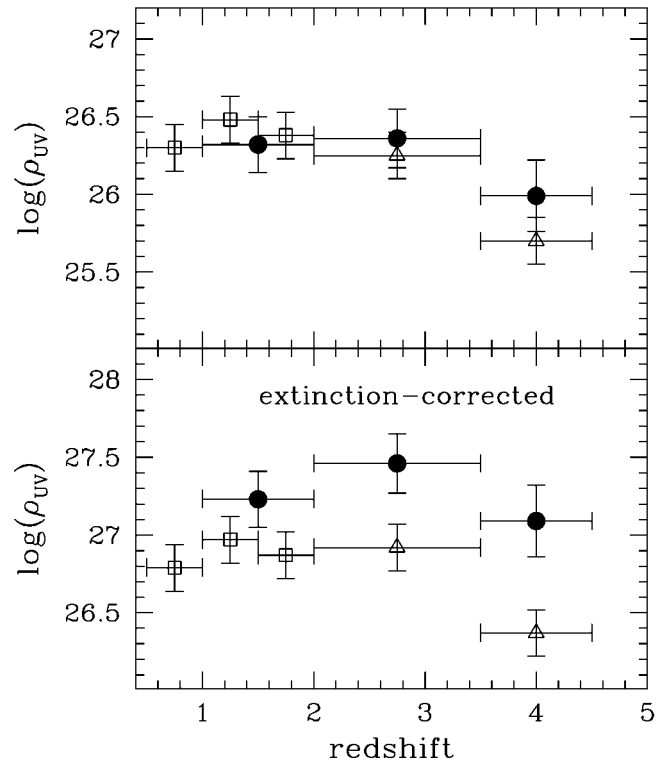
FIG. 1.—Redshift evolution of the comoving UV luminosity density (in log units of ergs s -1 Hz -1 Mpc -3 ), as sampled by the HDF-N galaxies. The apparent value of \rho_{(1500)} at 1500 Å, from the data in Table 1, is displayed in the upper panel, while its trend after correction for dust absorption is reported in the lower panel. Our results (filled circles) are compared with the Madau et al. (1998) 1500 Å data at z > 2 (triangles) and with the 2800 Å estimates of Connolly et al. (1997) at z < 2 (squares). Error bars on the points try to account for more realistic error estimates, including field-to-field variations (see Fontana et al. 1999) and errors induced by the unknown incompleteness of the sample studied.
