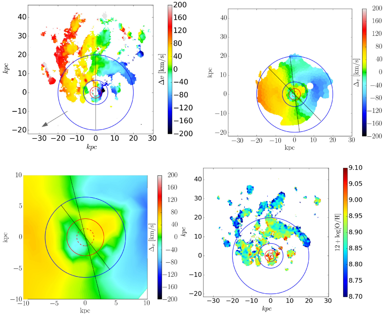
Figure 4. Gas (top left, H \alpha ) and stellar (top right) kinematics in JO171: ionized gas is present only in the northern part of the galaxy, and forms elongated tails that are being stripped from the galaxy. The arrow points towards the cluster centre (i.e. BCG). Stars are instead distributed in a symmetric pattern around the galaxy centre. The solid red circle delimits the spheroid and corresponds to the red solid line in Fig. 2, blue circles delimit the ring (also in blue in Fig. 2). The almost vertical line is the rotation axis of the stars, while the second inclined line ( \sim 37^\circ ) is the rotation axis of the central spheroid. The lower left panel shows a zoom in the central region of the stellar kinematics map, where the stellar spheroid counter-rotation appears. The bottom right panel shows the gas metallicity.
