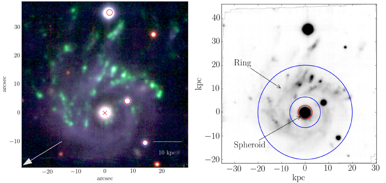
Figure 1. Left. RGB image of JO171 extracted from the MUSE data cube. The three bands correspond to the integrated flux in the Johnson I band (in grey colour), the integrated flux inside a 40 Å-wide band centred on H\alpha (thus including both the H\alpha emission and the continuum under H\alpha , here in green colour) and the integrated flux in the Johnson B band (blue in the image). Red circles indicate foreground stars that have been masked for the purposes of our analysis. The superimposed scale shows that 1 arcsec corresponds to 1.01 kpc at the galaxy redshift. North is up, East to the left. The arrow indicates the direction towards the brightest cluster galaxy (BCG). Right. A grey-scale image of the galaxy with superimposed a red circle enclosing the spheroid ( R_e ), and blue circles enclosing the ring (see the text).
