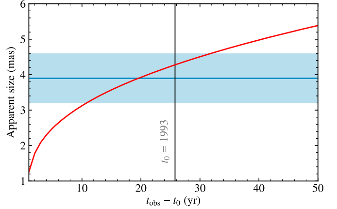
Figure 4. Apparent source size evolution. The red line shows the predicted apparent size evolution for a jet with parameters as those proposed by Law et al. (2018). The blue line and the lighter blue band show our measured apparent size and its 1\sigma uncertainty of \theta_s = 3.9 \pm 0.7 \text{ mas} . The gray vertical line marks the source age at the time of our observation, assuming that it originally exploded in 1993.
