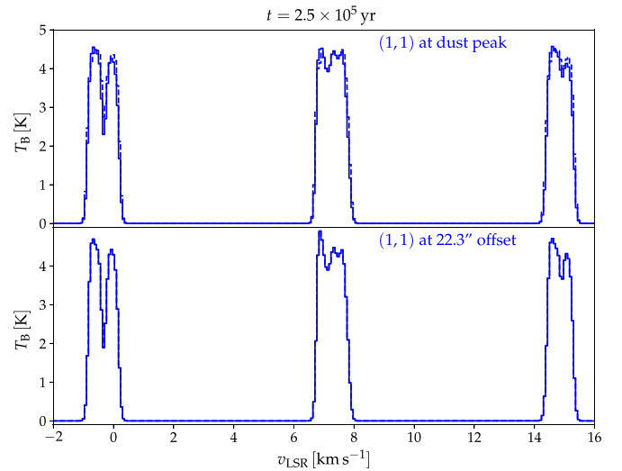
Figure F1. Simulated \text{NH}_3(1,1) spectra toward the dust peak (top panel) and an offset 22''.3 (bottom panel) away from the center, to be compared with the two spectra in Figure 2 of Crapsi et al. (2007). A beam of 4'' (close to the angular resolution of the VLA observations of Crapsi et al. 2007) has been assumed. The solid blue histogram is the spectrum obtained with the \text{NH}_3 abundance profile predicted by our model and shown in Figure 5, while the dashed blue histogram (only visible in the top panel, as in the bottom panel it coincides with the solid histogram) is the spectrum predicted assuming \text{NH}_3 constant abundance within the central 5000 au. Both spectra reproduce well the observed ones, within the observational uncertainties. It is then clear that \text{NH}_3(1,1) interferometric spectra of L1544 cannot provide constraints on the fractional abundance distribution of ammonia, unlike ALMA observations of \text{NH}_2\text{D}(1_{11}-1_{01}) (see Figure C1).
