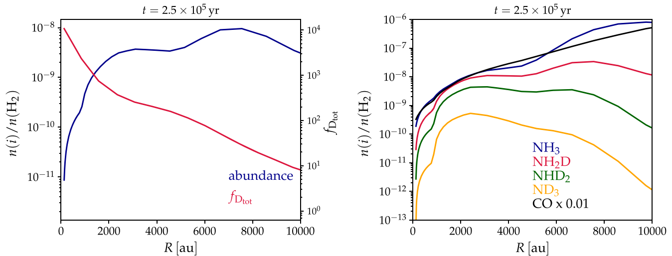
Figure 5. Left: model fractional abundance of \text{pNH}_2\text{D} (blue) and overall gas-phase depletion factor (red) at the best-fit time as a function of radius. Right: fractional abundances w.r.t. \text{H}_2 of normal and deuterated ammonia (colors, indicated in the figure), as well as of CO (multiplied by 0.01, black), at the best-fit time as a function of distance from the core center. The ammonia fractional abundances represent sums over the nuclear spin forms (ortho and para; also meta for \text{ND}_3 ).
