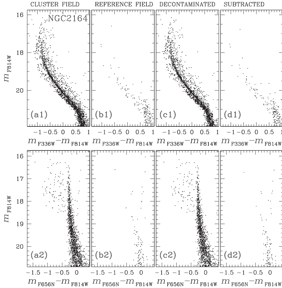
Figure 9. This figure illustrates the procedure to statistically subtract field stars from the cluster-field CMDs of NGC 2164. The upper and lower panels refer to the m_{F814W} versus m_{F336W} - m_{F814W} and m_{F814W} versus m_{F656N} - m_{F814W} CMDs, respectively. Panels (a1) and (a2) show the CMDs of stars in the cluster field, while the CMDs of stars in the reference field are plotted in panels (b1) and (b2). The decontaminated CMDs are shown in panels (c1) and (c2), while the subtracted stars are plotted in panels (d1) and (d2). See text for details.
