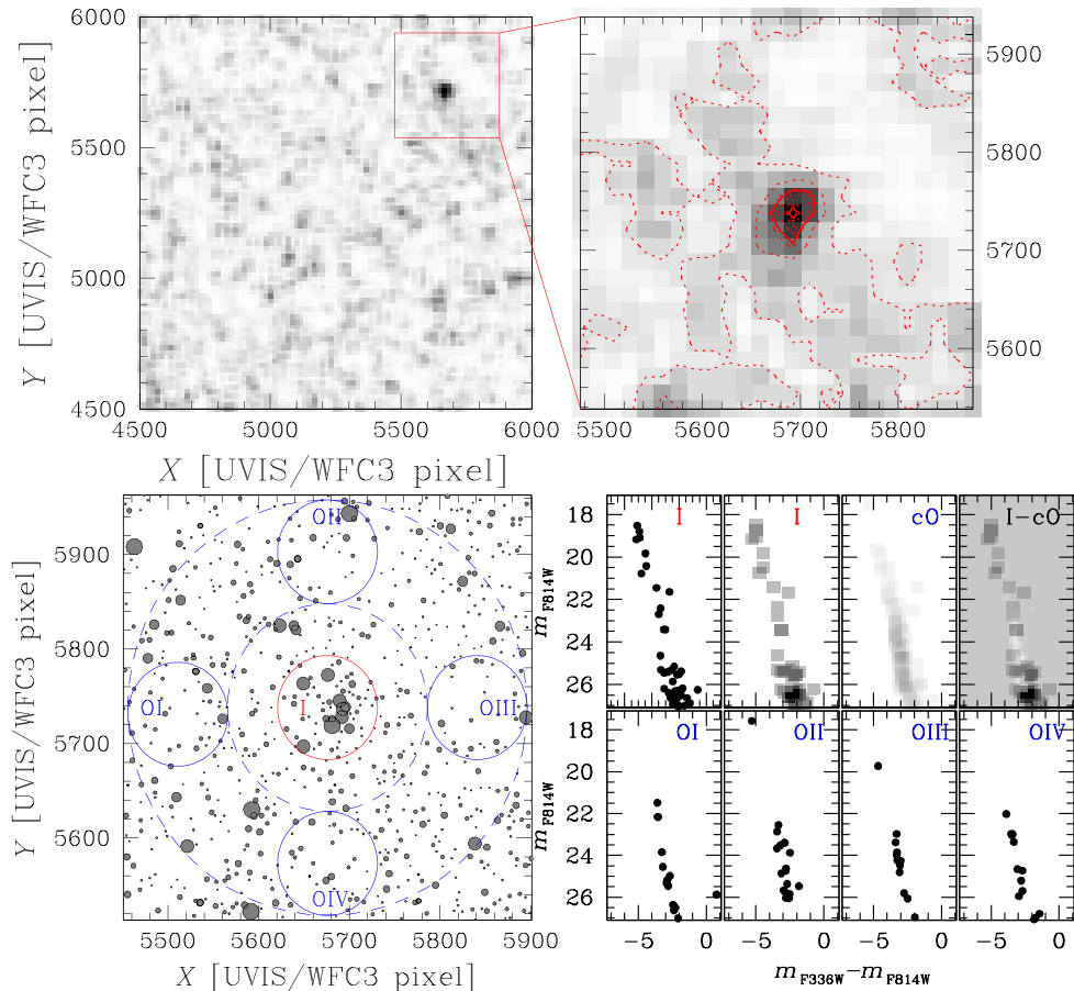
Figure A2. Map of stellar density for stars in a field of 1500 \times 1500 UVIS/WFC3 pixels ( 1.0 \times 1.0 \text{ arcmin}^2 ) south-east of NGC 330 (upper left-hand panel). The upper right-hand panel shows a zoom-in of the upper left-hand panel plot in a region centred on the newly discovered star cluster. The contours of stellar density are represented with red lines. The lower left-hand panel shows a map of stars around the newly discovered star cluster. The red circle marks the inner field, I, while the region between the two dashed circles is indicated as the outer field. The four subregions of the outer field (OI, OII, OIII, and OIV) are marked with blue-continuous fields. The m_{F814W} versus m_{F336W} - m_{F814W} CMDs of stars in the fields I and OI–OIV are shown in the lower right-hand panels, where we also plotted the Hess diagram of stars in the fields I and O and the Hess diagram of the corresponding difference. See text for details.
