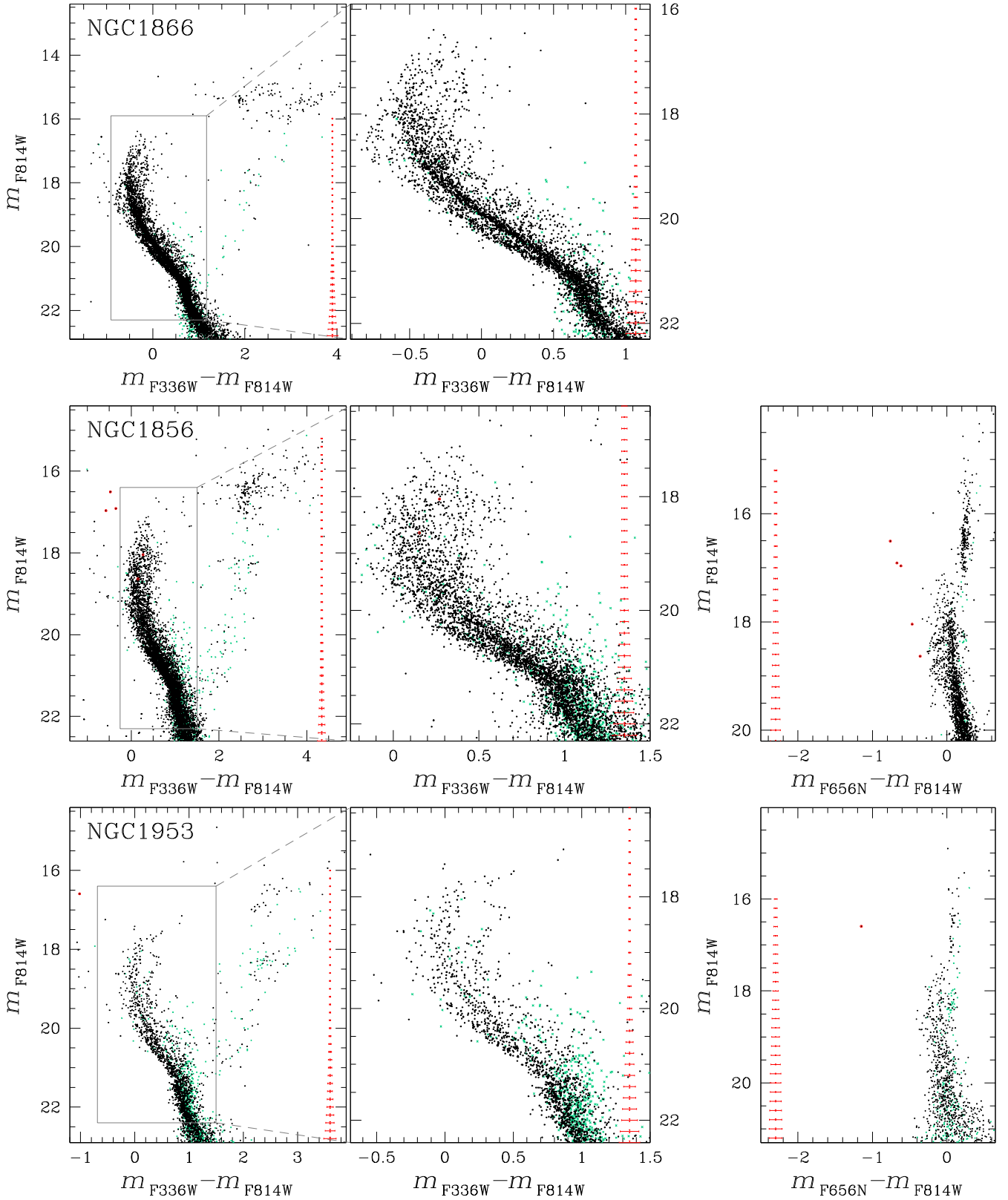
Figure 4. As in Fig. 2 but for NGC 1866, NGC 1856, and NGC 1953. Photometry in the F656N band is not available for NGC 1866.
