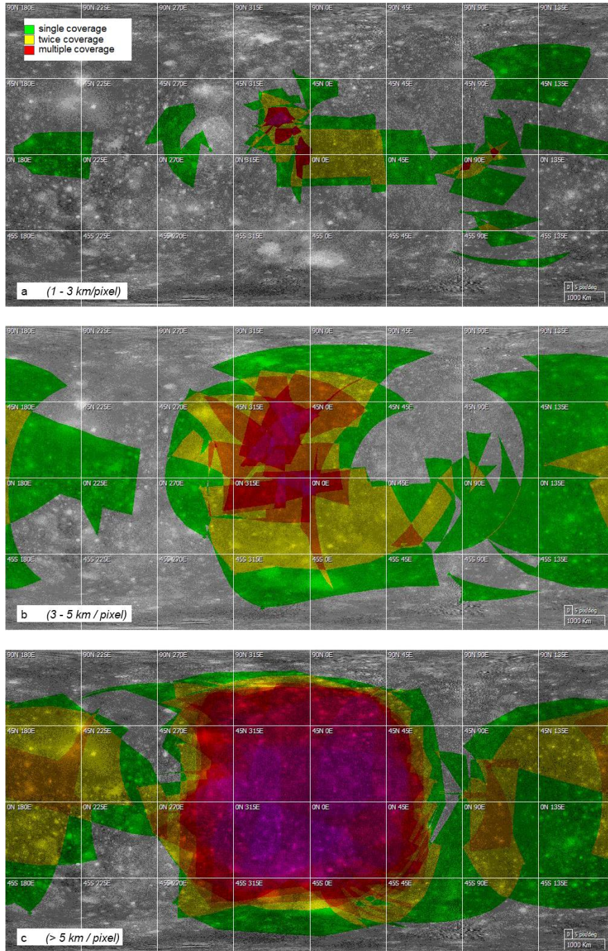
Figure 5: MAJIS coverage during the Callisto flybys (CReMA 3.0) by observations with spatial resolutions a) between 1 and 3 km / pixel, b) 3 and 5 km / pixel and c) > 5 km / pixel with the overlap of MAJIS observations indicated. The Figure was prepared using the Mission Analysis and Payload Planning System (MAPPS) of ESA (Van Der Plas and Nespoli, 2016).
