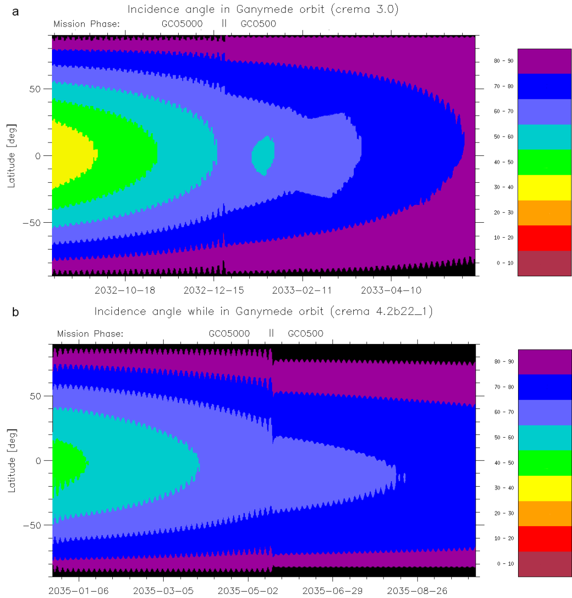
2 Figure 2: Development of the illumination conditions (incidence angle ( ^{\circ} ) during GCO5000 and 3 GCO500: a) based on CReMA 3.0 and b) CReMA 4.2b22.1 across the full range of latitudes on 4 Ganymede's surface.
