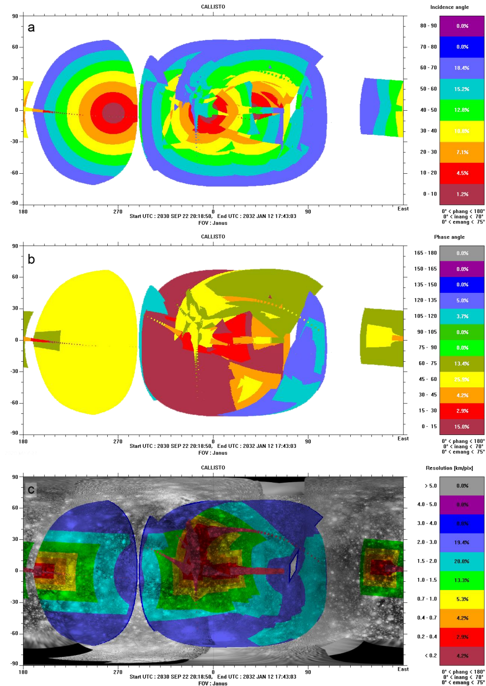
1 2 Figure 3: JANUS coverage (nadir-looking only) during the Callisto flybys (CRema 3.0): a) 3 incidence angle, b) phase angle and c) spatial resolution overlaid onto the global Galileo/Voyager 4 base map provided by USGS.
