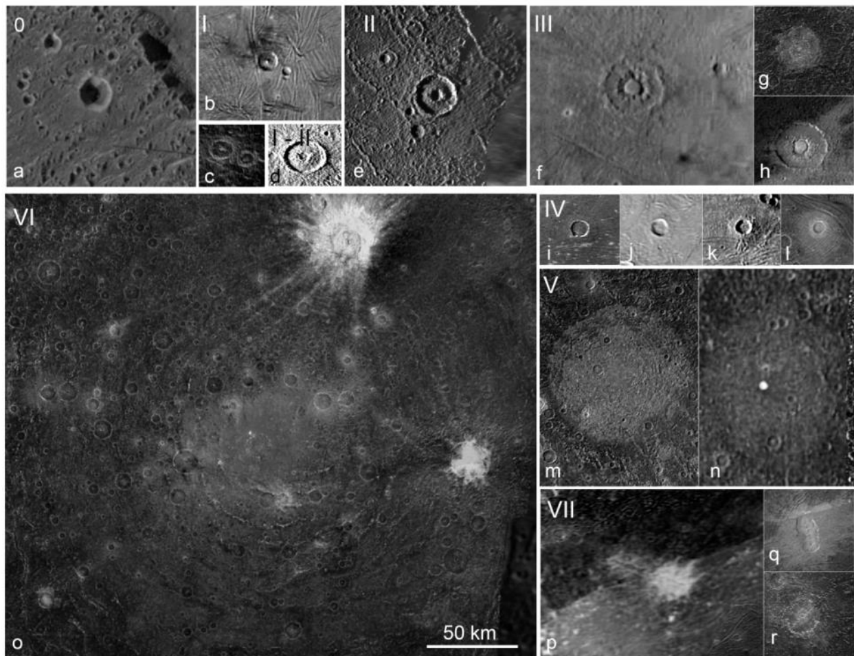
Figure 14: Examples of impact crater morphologies (category 0 - VI) on Ganymede (G) and Callisto (C): a) simple bowl shape (0), b) and c) central peak (I), d) and e) central pit (II) partly showing the transition from peak to pit (I – II), f) – h) central dome (III), i) – l) pedestal (IV) and m) – n) palimpsest (V); o) multiring impact basins; and p) – r) catenae (VII) with the RoI IDs b) (G) #4.1.1, c) (C) #4.1.1., d) (G) #4.2.4, e) (G) #4.2.1, f) (G) #4.3.6, g) (C) #4.3.2, h) (G) #4.3.2, i) (G) #4.4.5, j) (G) #4.4.3, k) (G) #4.4.11, l) (G) #4.4.6, m) (G) #4.5.2 n) (C) #4.5.1 o) (C) #4.6.1 (scale bar fits to all images), p) (G) #4.7.3, q) (G) #4.7.4, and r) (C) #4.7.1.
