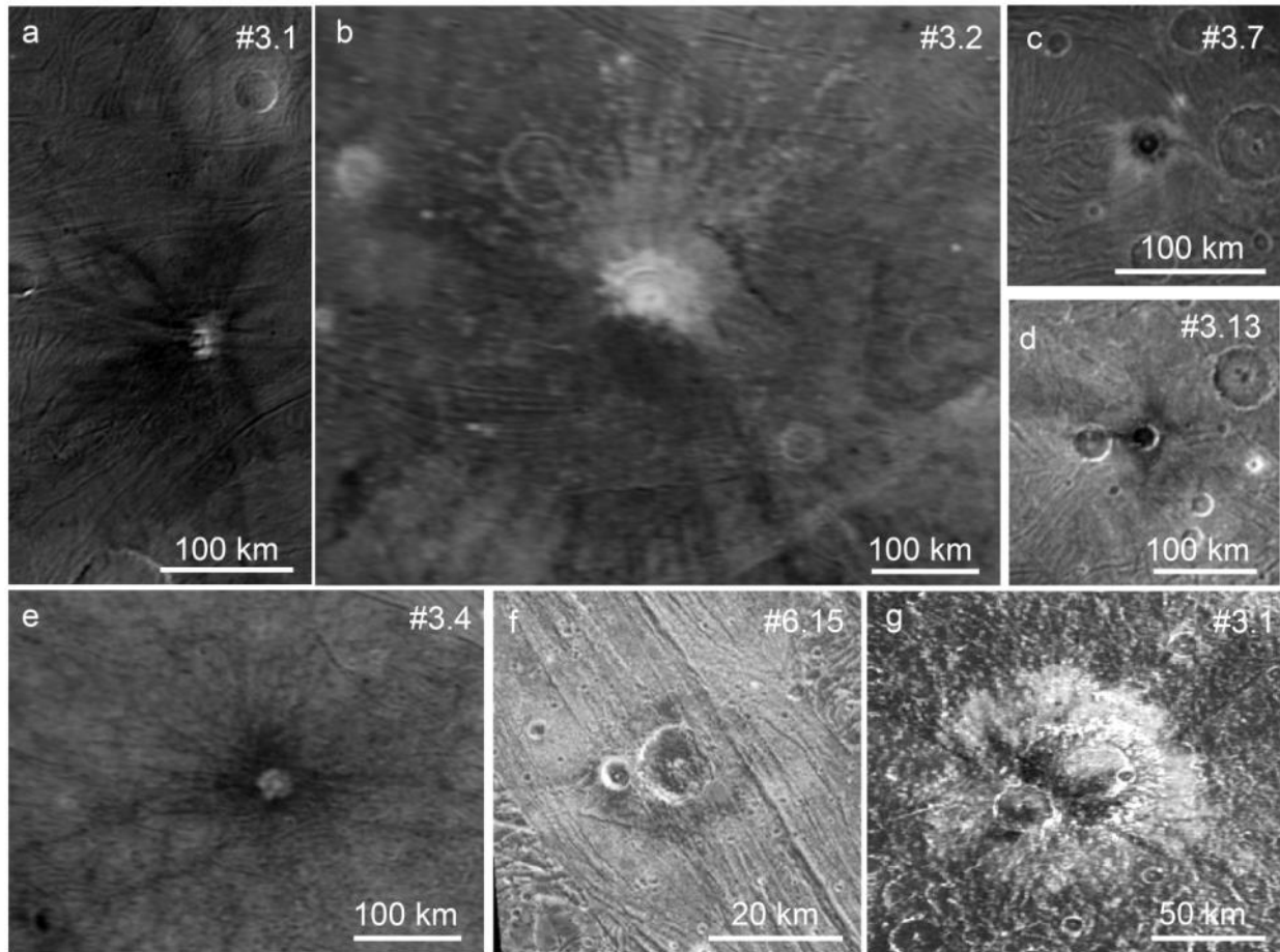
Figure 12: Examples of dark ray, floor and halo craters on Ganymede (a - f) and Callisto (g) proposed to be observed during the JUICE mission. Some of very small dark impact craters are incorporated in RoIs of other categories such as f) the small impact crater Nergal (38.6°N/159.5°E) in Byblos Sulcus (ID #6.1.5).
