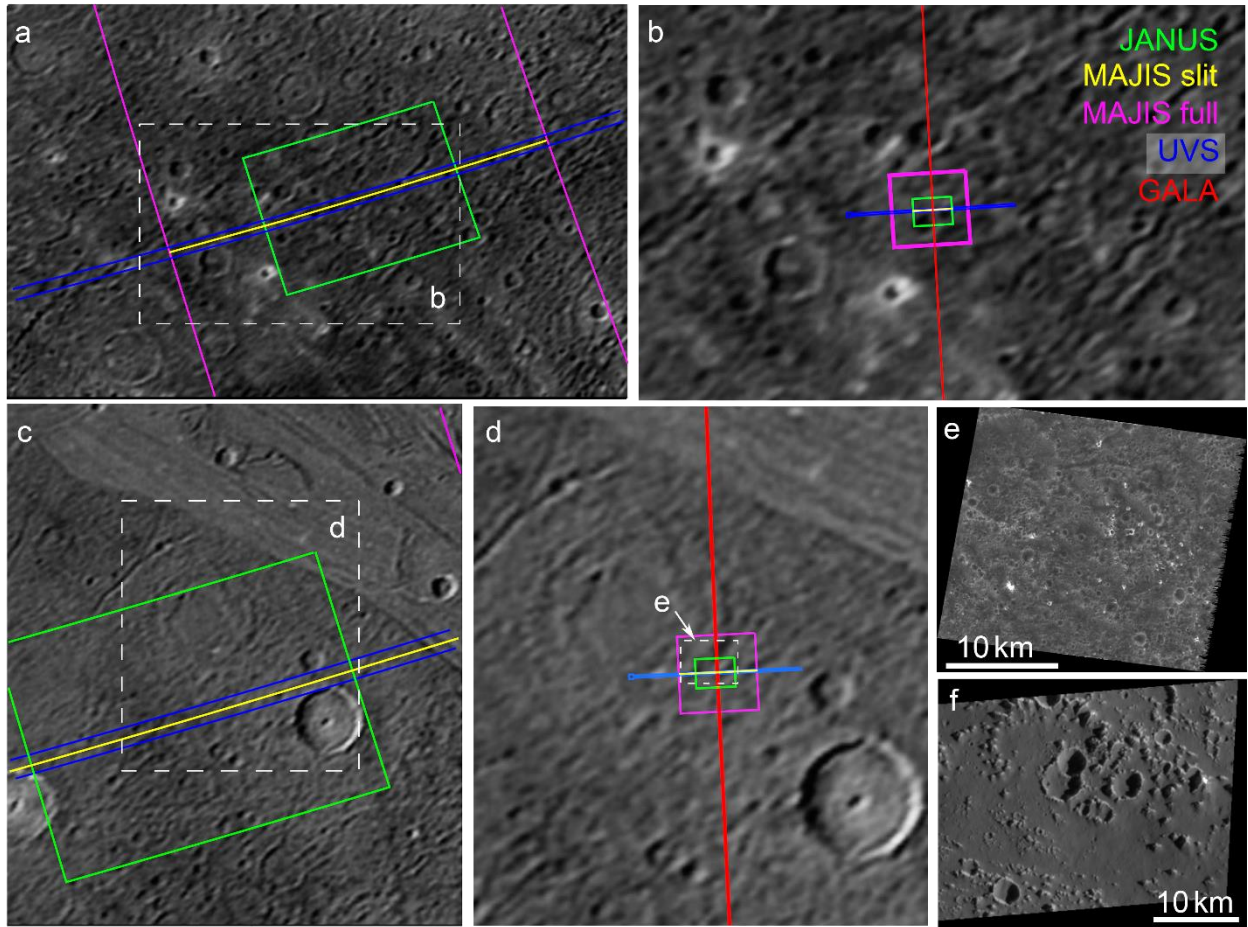
Figure 19: Examples of selected target regions for the investigation of the ancient dark terrain: 1) portion of Nicholson Regio selected for RoI #7.5 overlaid by single footprints possible during a) GCO5000 and b) GCO500 and 2) portions of Nicholson Regio surrounding an ancient palimpsest selected as RoI#4.5.14 (as an example of dark terrain seen in RoIs of other categories) overlaid by possible footprints during c) GCO5000 and d) GCO500, which include e) the portion of Nicholson Regio on Ganymede observed by Galileo SSI ( \sim 10.6^{\circ}\text{S}/34.6^{\circ}\text{E} ; \sim 25 m/pixel) in comparison with f) the dark terrain on Callisto ( \sim 22^{\circ}\text{N}/\sim 218^{\circ}\text{E} ; \sim 900 m/pixel) located in the southern portion of the ancient impact basin Asgard, which is covered by RoI #7.1. Please note that GALA will not operate during GCO5000.
