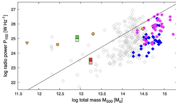
Figure 6. Scaling relation of 150 MHz radio power ( P_{150} ) versus total mass ( M_{500} ) for cluster radio relics (including candidates) from Jones et al. (2023, blue diamonds), including double relics from de Gasperin et al. (2014, pink diamonds), brightest cluster radio galaxies from Pasini et al. (2022, grey symbols), and our sample of ORCs and similar radio shell systems (see Table 3). ORCs are shown in orange, the Cloverleaf system in green, and the Physalis system in red. For the latter two, we show the system radio power (dark squares) as well as the approximate radio power of the shells alone (light squares; estimated to be around 60 per cent). The black line indicates P_{150} \propto M_{500}^{5/3} , which corresponds to self-similar scaling assuming the same fraction of merging energy going into the radio power (e.g. de Gasperin et al. 2014).
