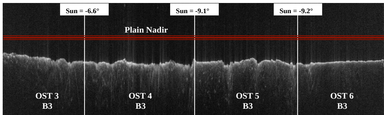
Fig. 3.1.1 (MARSIS Radargram, first Tx Bands)
