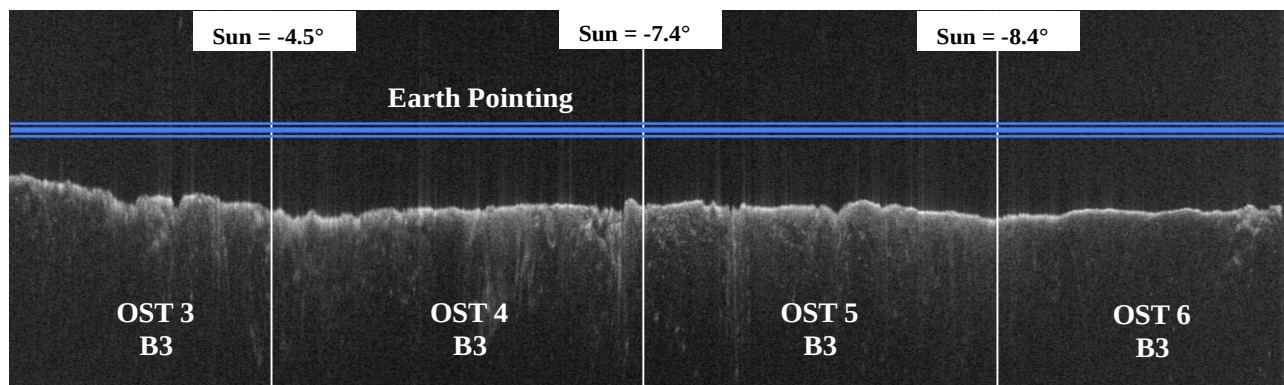
Fig. 3.2.1 (MARSIS Radargram, first Tx Bands)
