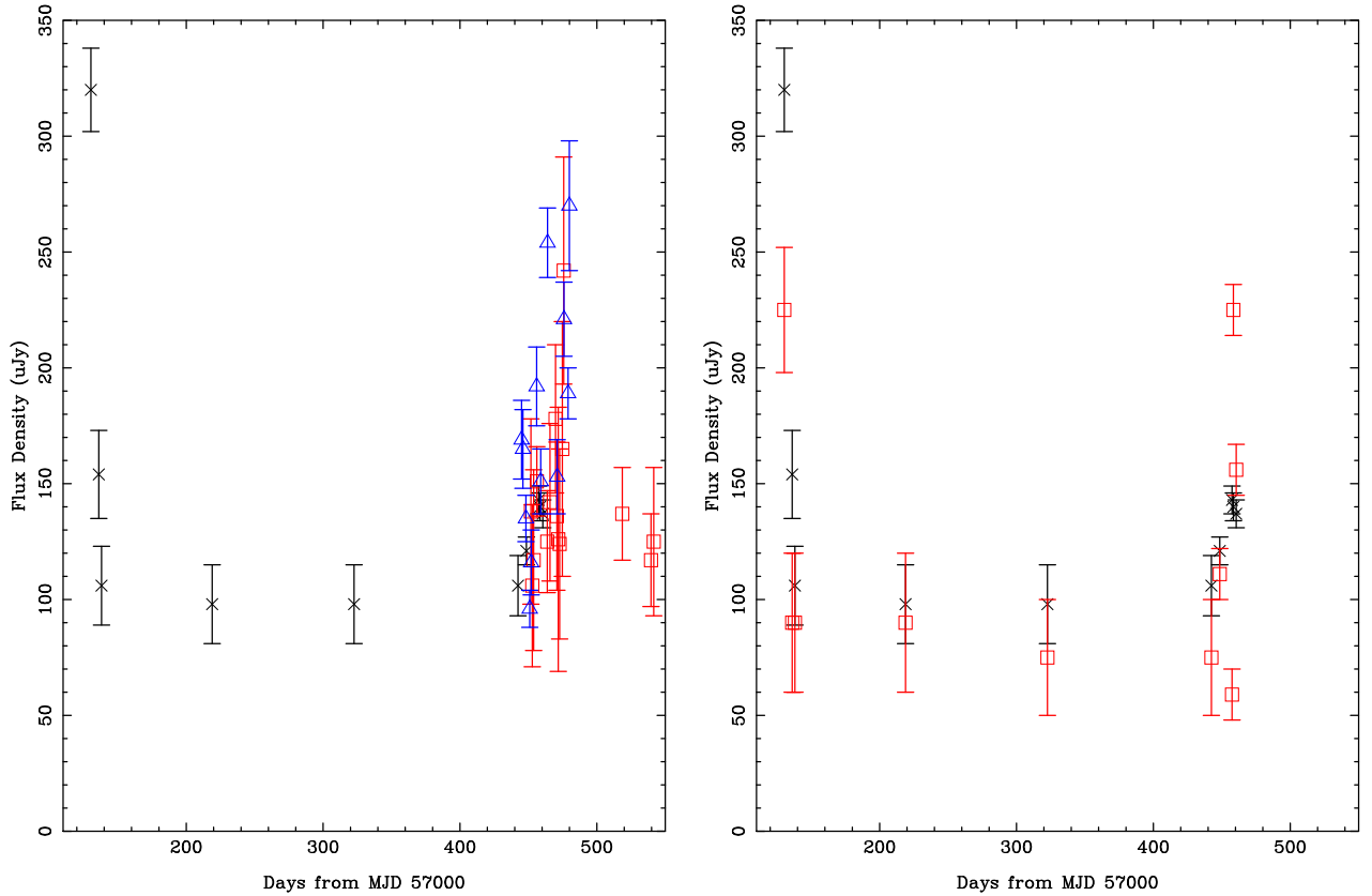
Figure 1. Left-hand panel: radio light curve at 5.5 GHz. Black crosses denote ATCA observations, blue triangles JVLA observations, and red squares VLBA, e-MERLIN and EVN. Right-hand panel: radio light curve from the ATCA data at 5.5 GHz (black crosses) and 7.5 GHz (red squares).
