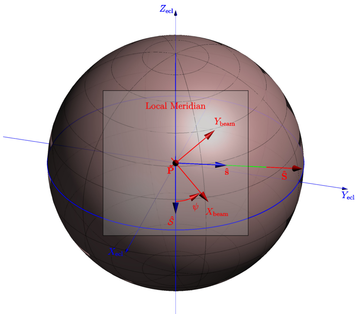
Figure 2: The Tangent Reference Frame (blue) and the Beam Reference Frame (red). The view is for an observer looking from the top of the pointing direction. The figure defines also the \psi angle.
