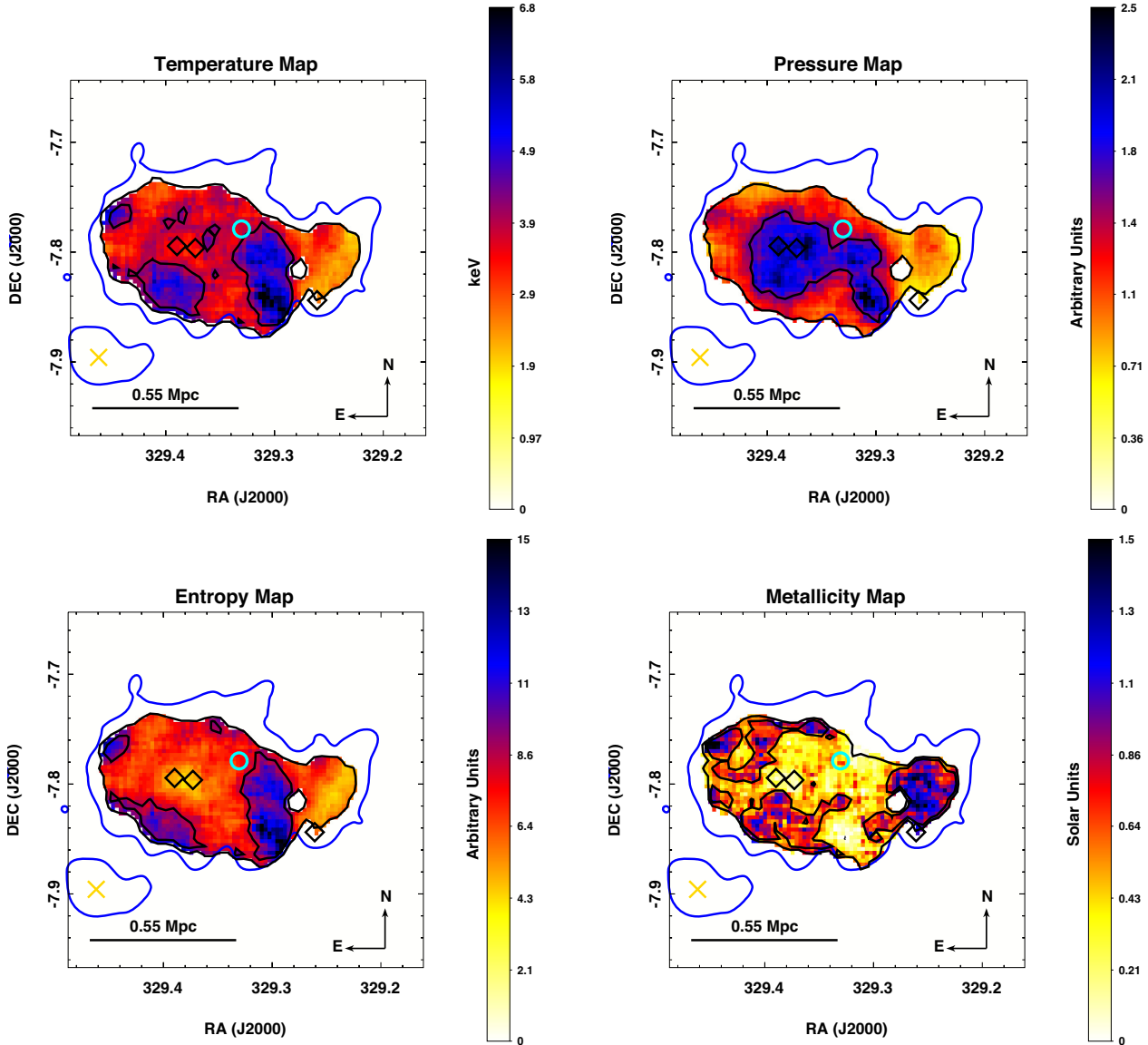
Figure 8. X-ray spectral maps. The open circles in cyan show the position of JO69, a jellyfish galaxy. The open black diamonds indicate where the BCGs are located, and the yellow cross marks the position of a foreground star. The blue contour shows the X-ray emission from XMM-Newton . All the maps show that A2399 is a disturbed cluster with a western clump that resembles a bullet.
