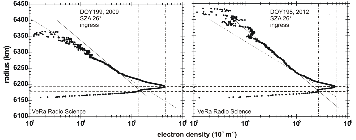
Figure 31: two VeRa electron density profiles observed at solar minimum (panel a) and solar maximum (panel b). Both layers V1 and V2 appear stronger and more pronounced at solar maximum than at solar minimum (dashed-dotted vertical lines). There is no obvious change in the altitudes of the V1 and V2 layers (dashed horizontal lines). The slope of the diffusion region is also steeper at solar maximum (solid line) then at solar minimum (dash-dotted inclined line). Figure courtesy VEX VeRa team. See comment by reviewer #1.
