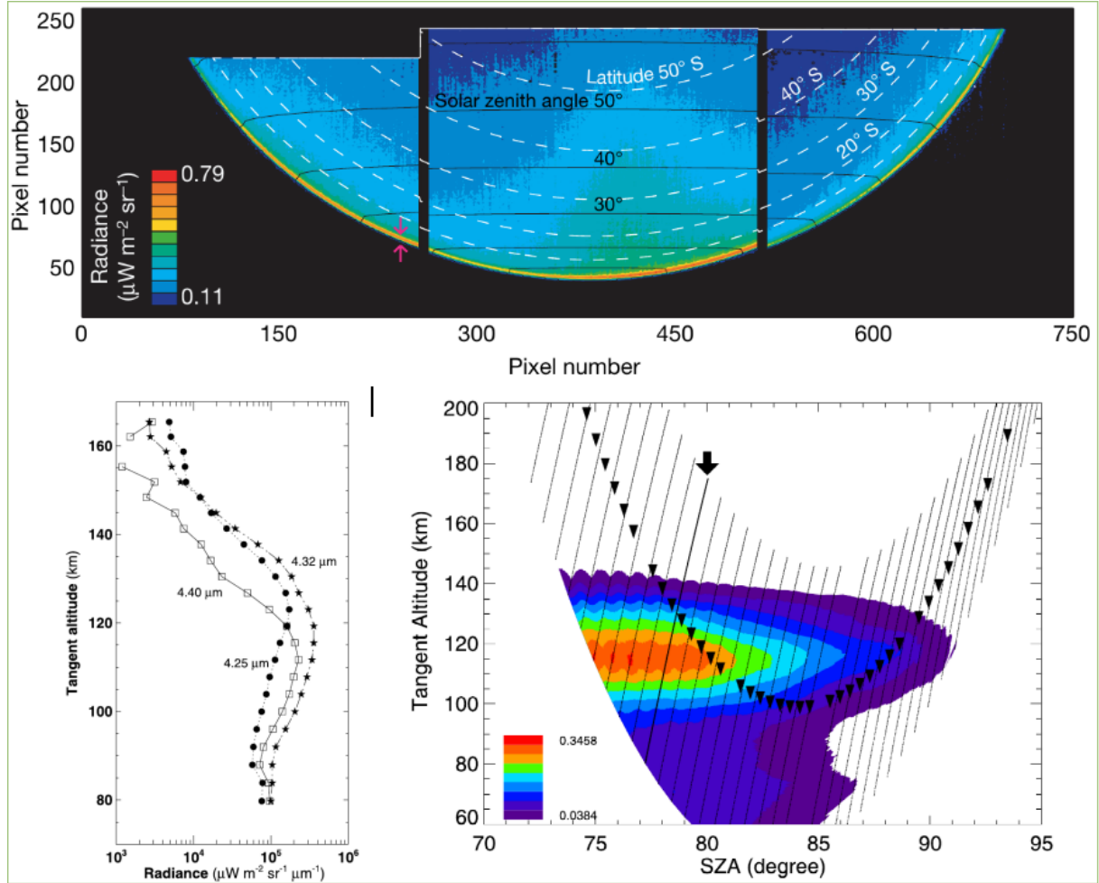
Figure 8: Top: Composition of three VIRTIS-M spectral data cubes during Orbit 25, at 4.33 μm, showing nadir and limb emission levels, with variations not totally explained by the expected SZA changes (after Drossart et al., 2007). Bottom-Left: Limb profiles at three wavelengths obtained by combining individual adjacent pixels in one of the cubes of the VIRTIS-M image in orbit 25, in this case with spacing around 4 km in the vertical. Bottom-Right: Set of successive slit-frames of VIRTIS-M from its “spectral mode” during one pericenter observation. Triangles show the center of the slit, where VIRTIS-H data are also available. The emission map only uses VIRTIS-M data (after Gilli et al., 2009). SEE comments for reviewer #1.
