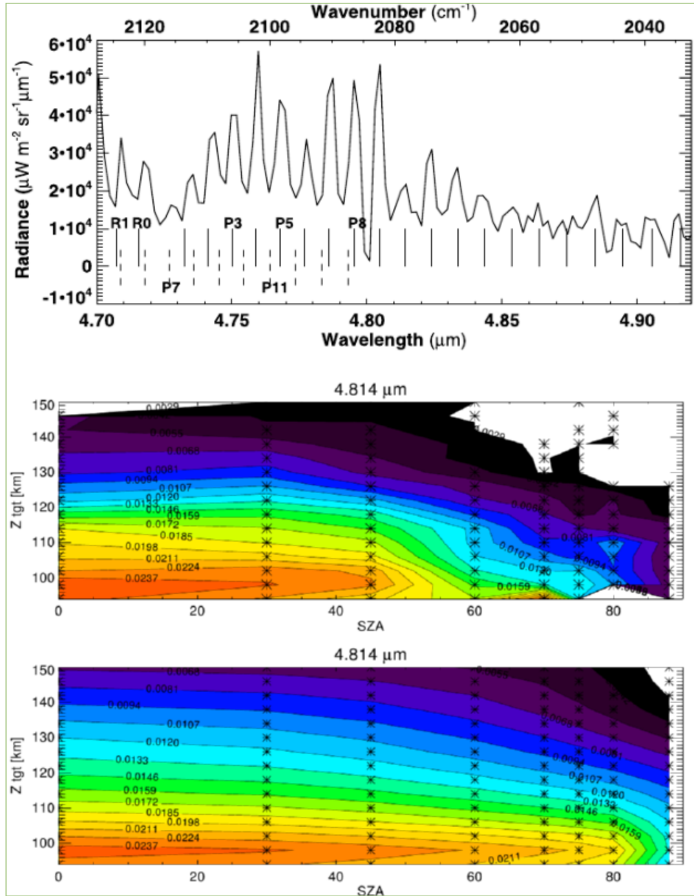
Figure 9: Top: VIRTIS-H limb spectrum at 4.7 \mu\text{m} , taken at an altitude around 85 km and SZA=60°, showing individual lines of the CO fundamental (dash markings) and first hot bands (solid markings) (after Gilli et al., 2009). Middle and Bottom panels: Observations (VIRTIS-H) and model simulations of the altitude/SZA cross section of the CO emission at 4.7 \mu\text{m} (at 4.81 \mu\text{m} ); observations combine data from many orbits and become very noisy at high SZA (after Gilli et al., 2015). See comment by reviewer #1.
