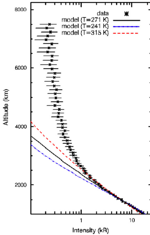
Figure 26: Lyman- \alpha intensity profile observed with SPICAV (stars) and comparison with the best fit profile ( T=271 K) to the measurements below 2000 km (solid line). Intensity profiles at 241 K and 315 K are shown in blue and red, respectively. The scale height of the observed profile is much brighter than the best fit above 4000 km as a consequence of the presence of hot H atoms (from Chauffray et al., 2012b)
