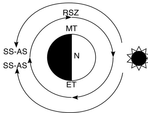
Figure 18: Illustration of the major components of the global circulation of the Venus upper atmosphere. SS-AS (subsolar-to-antisolar), RSZ (retrograde superrotating zonal), ET (evening terminator), MT (morning terminator) (from Brecht et al., 2011).
