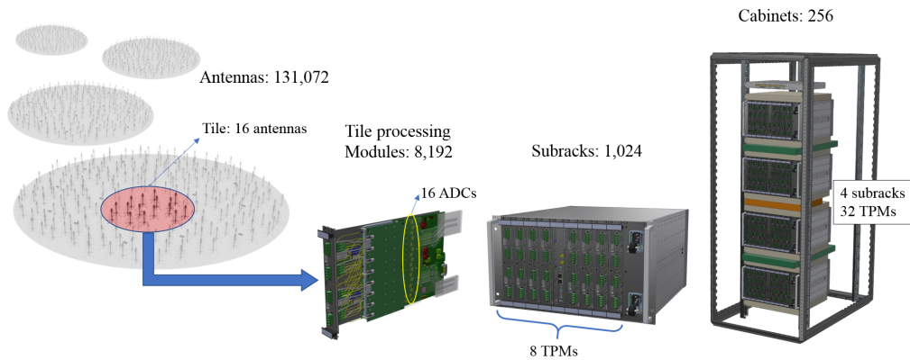
Fig. 1 Hierarchical structure of the SPS physical implementation. Each tile (16 antennas) is digitized and processed in a tile processing module (TPM), eight TPMs are housed in a subrack, and four subracks (32 TPMs) are hosted in a cabinet.
