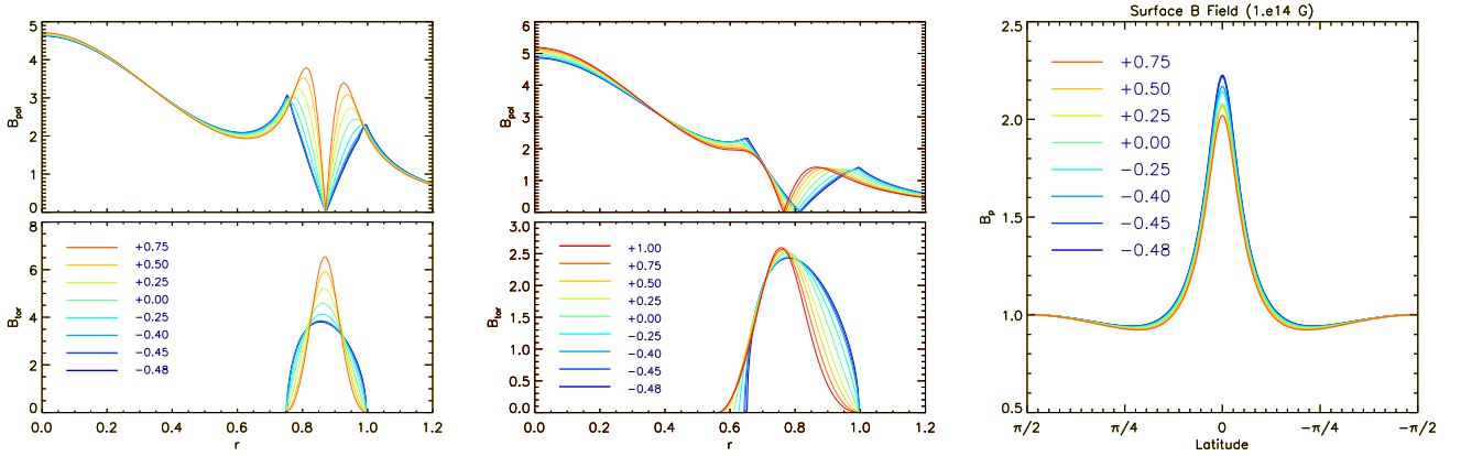
Figure 6. Left-hand panel: strength of the poloidal magnetic field (top) and toroidal magnetic field (bottom) inside the star, on the equatorial plane, as a function of r , normalized to R_{\text{NS}} , for models corresponding to the maximum of \mathcal{H}_{\text{tor}}/\mathcal{H} , for various values of \zeta . Middle panel: strength of the poloidal magnetic field (top) and toroidal magnetic field (bottom) inside the star, on the equatorial plane, as a function of r , for models corresponding to B_{\text{tor}}^{\text{max}}/B_{\text{pol}}^{\text{max}} = 0.5 . Right-hand panel: strength of the magnetic field at the surface for models corresponding to the maximum of \mathcal{H}_{\text{tor}}/\mathcal{H} . In all cases the strength is normalized to the surface value at the pole.
