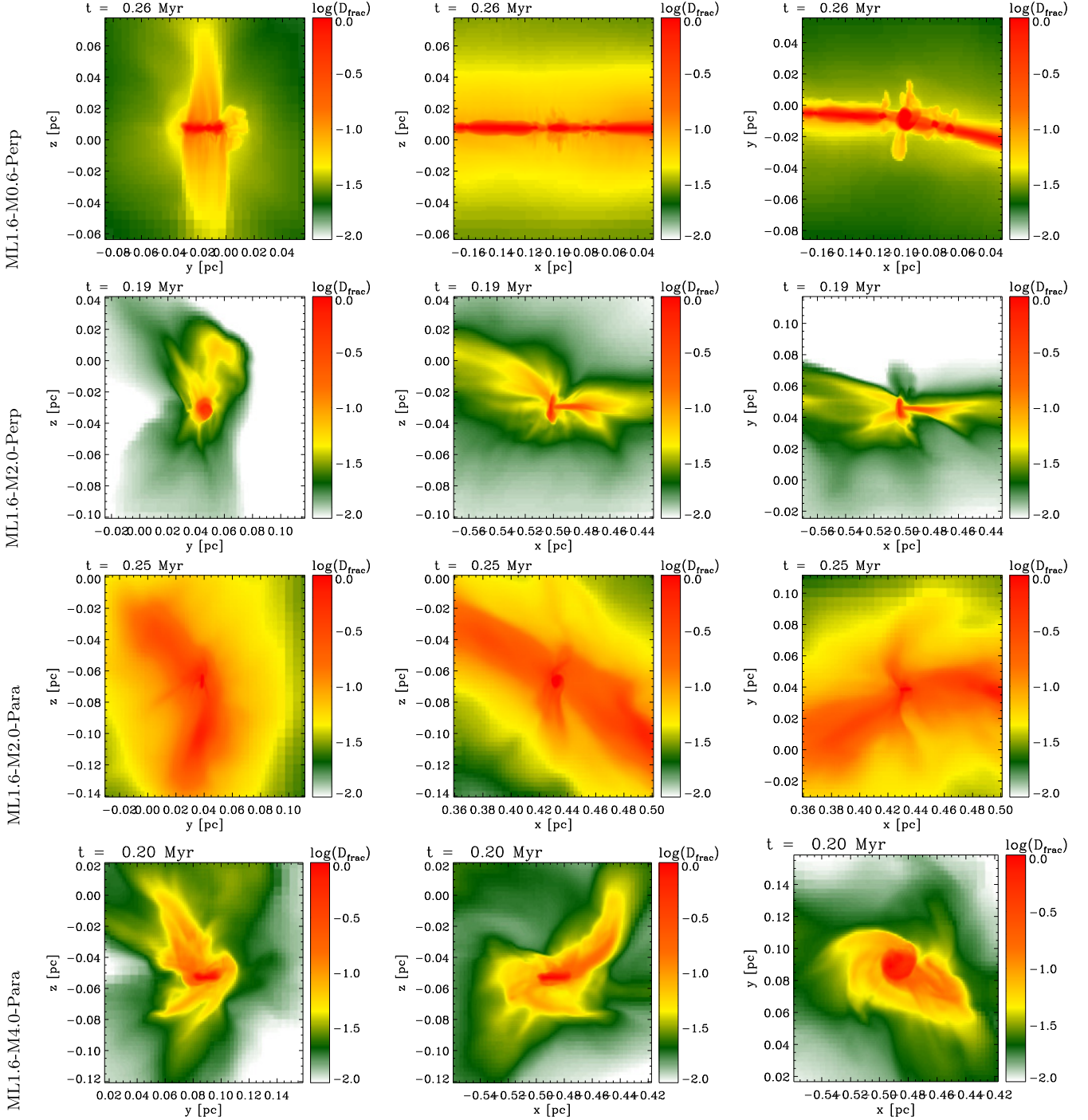
Figure 7. Deuterium fraction of selected cores in different filaments at the end of the simulation. Shown is the deuterium fraction along different directions. Integration length in all cases is l = 0.2 pc. The previously mentioned high-density channels are also regions of greatly enhanced deuterium fraction, giving rise to accretion of highly deuterated material.
