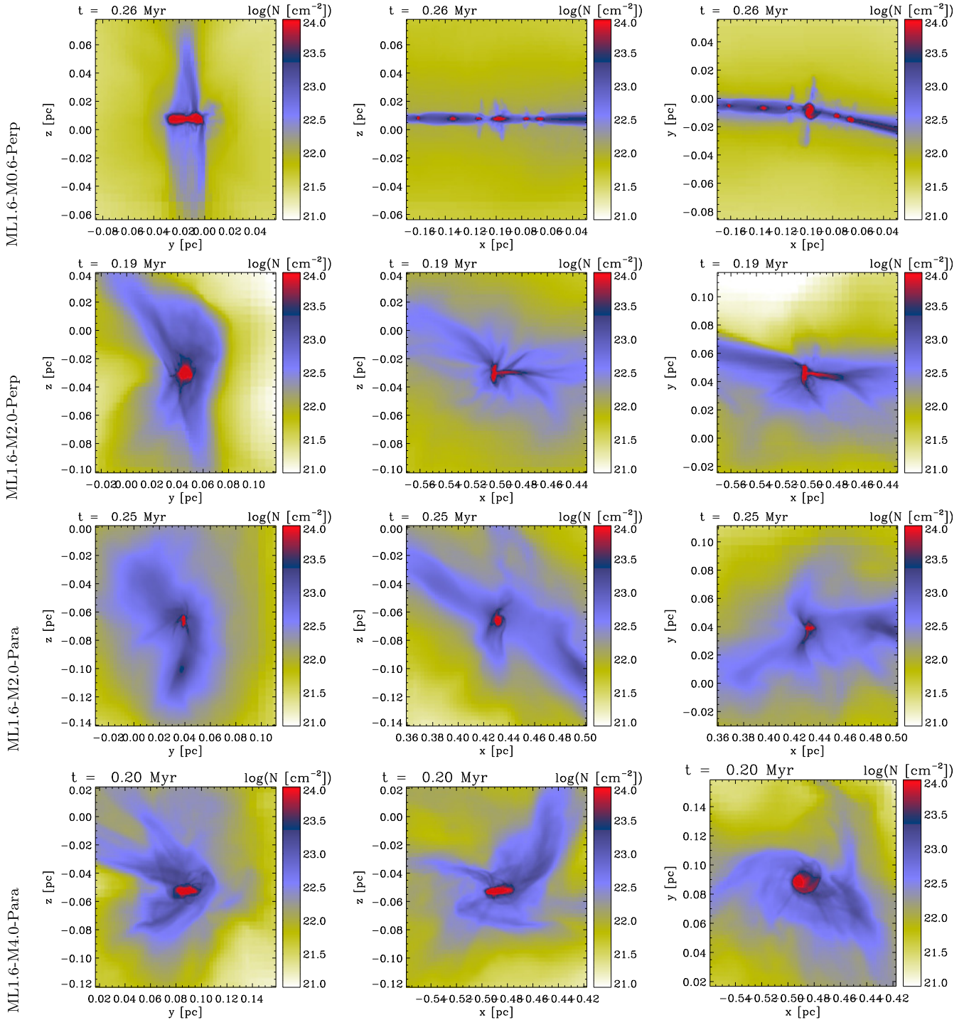
Figure 6. Zoom-in to selected cores in different filaments at the end of the simulation. Shown is the column density along different directions. Integration length in all cases is l = 0.2 \text{ pc} . All cores reveal an oblate geometry. Only with initially supersonic turbulence, the core environment becomes highly irregular and dynamic. Note the finger-like structures of enhanced column density near the cores.
