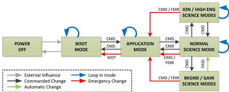
Fig. 87 Strofio Mode Transition Diagram
