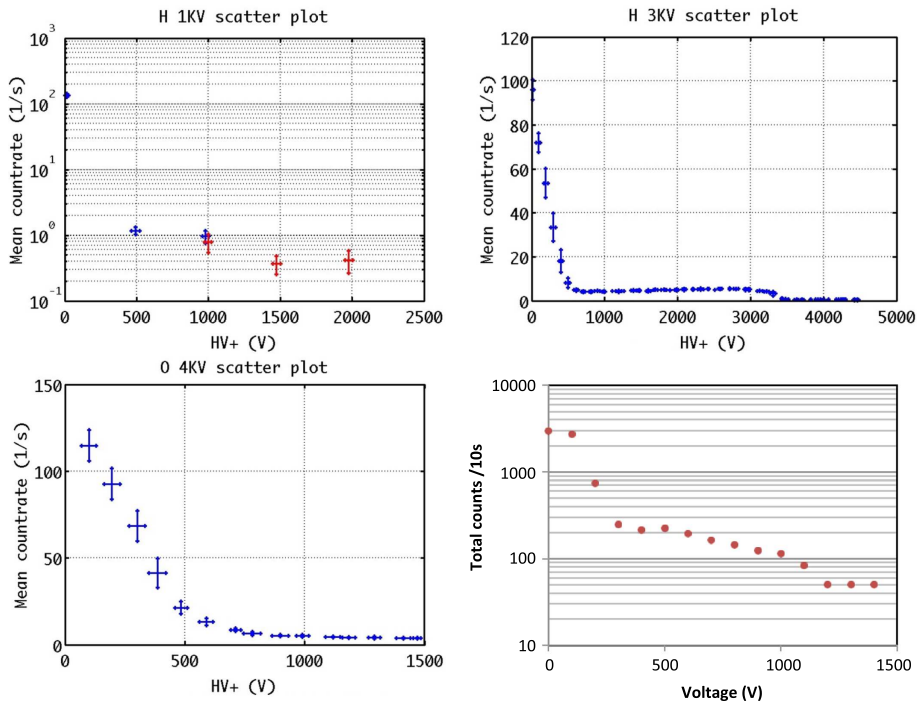
Fig. 46 Counts vs PP applied. FS test: 1-keV (above left) and 3-keV (above right) H + 4-keV O + (below left). PFM test: 1-keV H + (below right)
