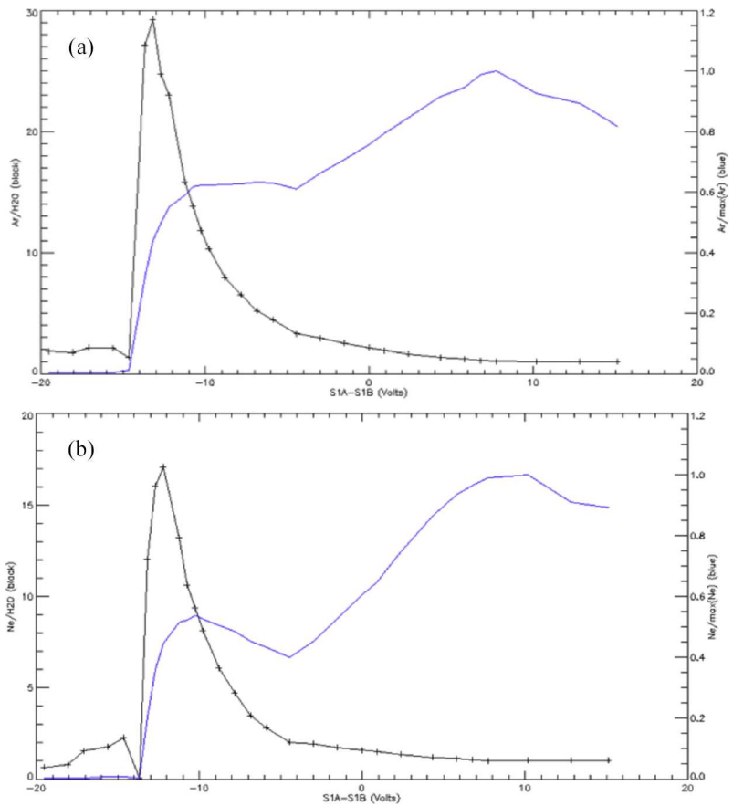
Fig. 62 Velocity filter effects on Strofiio response for (a) Ar and H 2 O, (b) Ne and H 2 O
