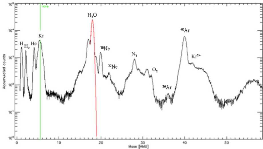
Fig. 56 Strofi mass range for two turns
