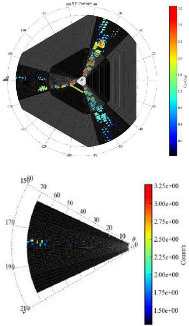
Fig. 74 (left) MIPA calibration with 500 eV N^+ in D0 sector, (right) Full coverage at 500 eV N^+ . From BC-SRN-TR-40020-01-00 _MIPA FM Calibration Report
