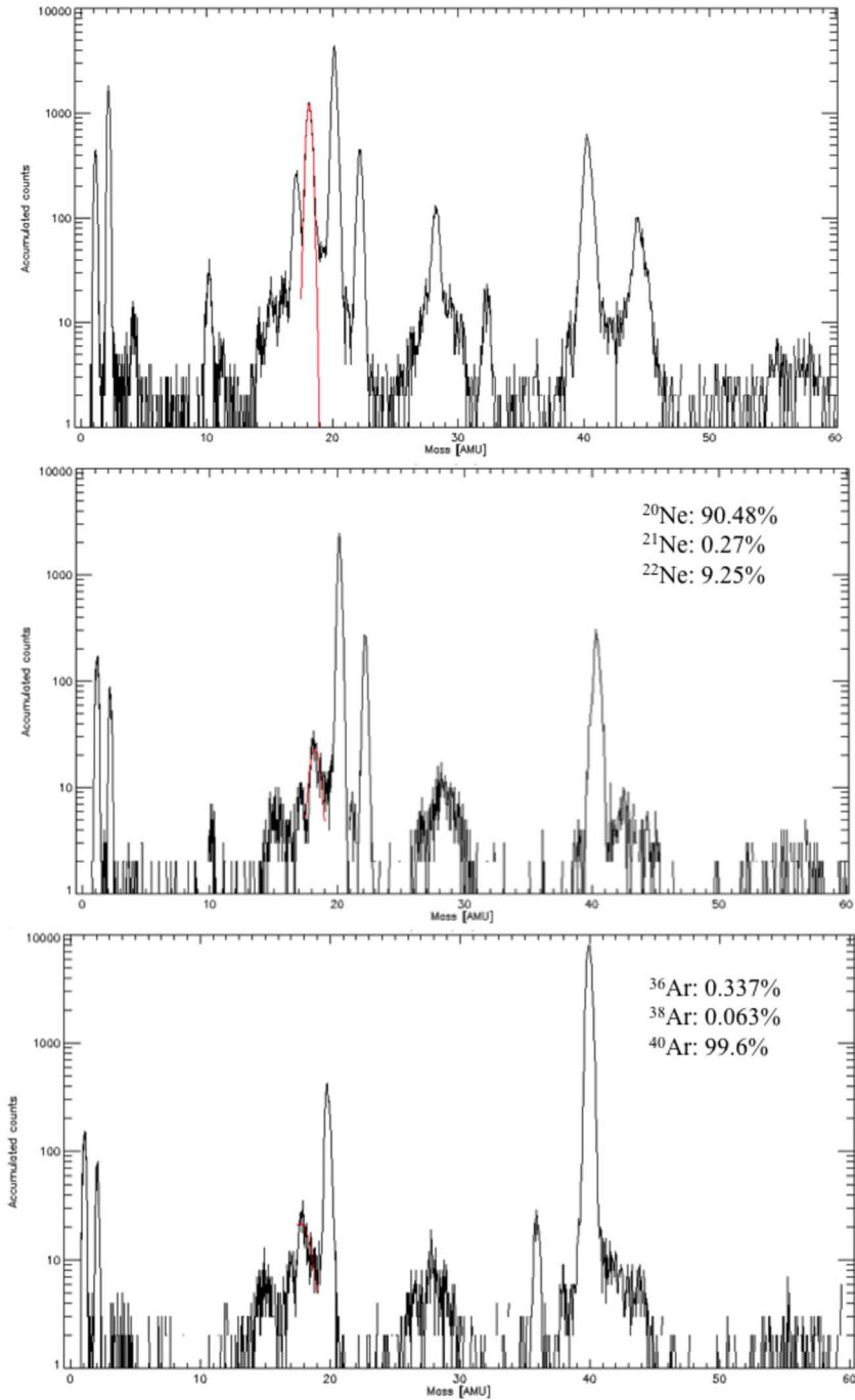
Fig. 55 Top: Strofi mass resolution without a velocity filter. Middle: mass resolution of Ne isotopes with a velocity filter. Down: mass resolution of Ar isotopes with a velocity filter
