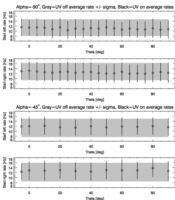
Fig. 63 Results of UV contamination tests for Strofi MCPs
