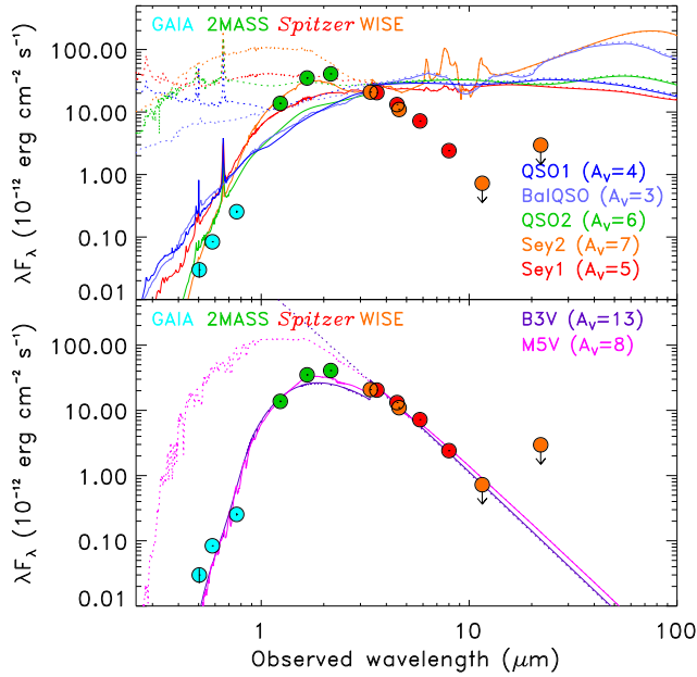
Figure 6. Spectral energy distribution of AX J1714.1 – 3912 (full circles: GAIA in cyan, 2MASS in green, Spitzer in red and WISE in orange). The lines represent various templates normalized at the observed 3.6\mu\text{m} flux with no reddening (dotted) or with different amounts of reddening (solid), as annotated, applied to reproduce the observed optical-NIR SED. Templates of various types of AGN are shown in the top panel (Polletta et al. 2007), and of a B and M-type star (Kurucz 1993) in the bottom panel .
