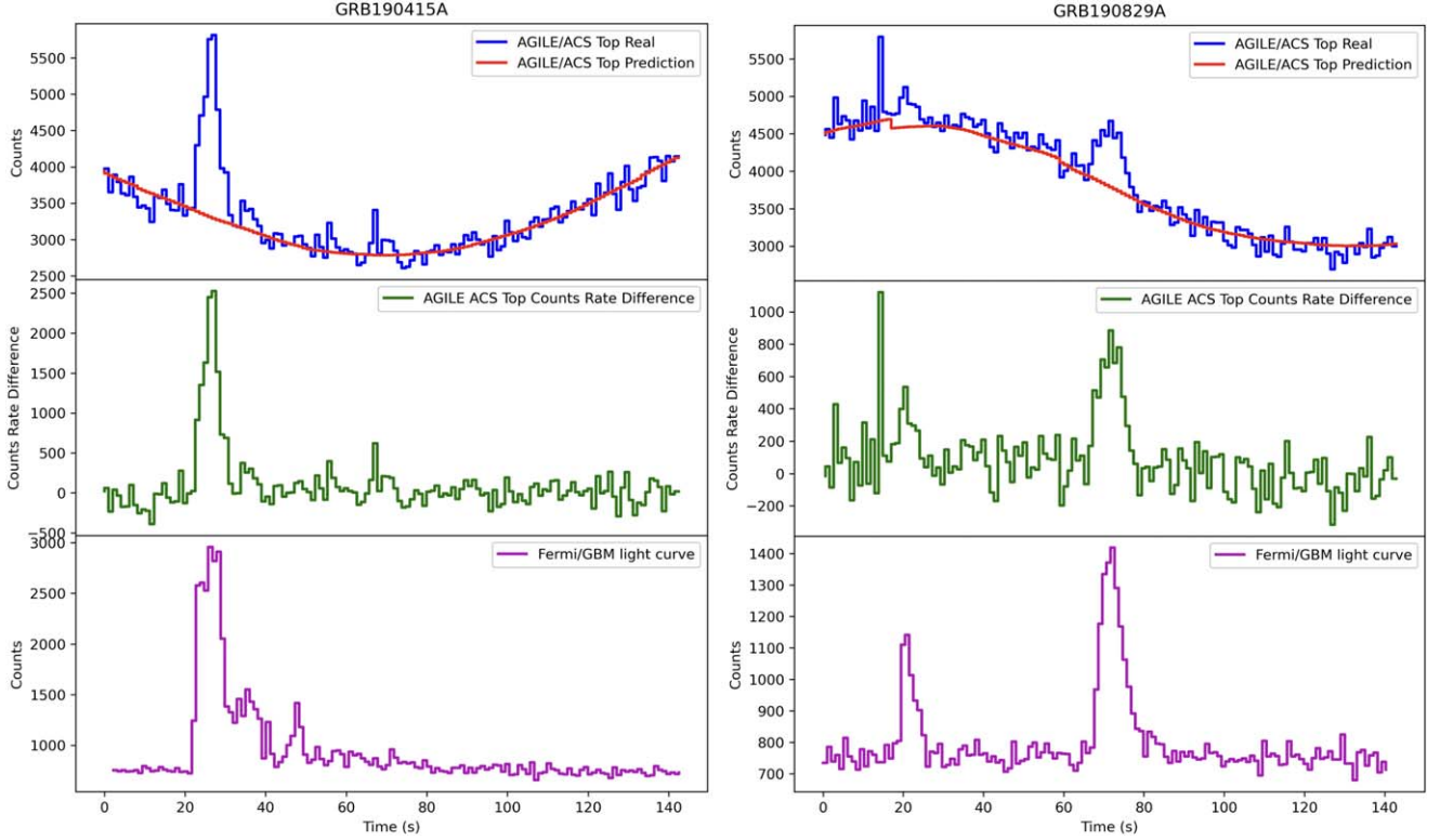
Figure 9. Comparison between light curves of the GRB190415A and GRB190829A acquired by the AGILE/ACS top panel (50–200 keV) and the Fermi/GBM (50–300 keV). The trigger time of the GRBs is 20 s from the start of the light curves.
