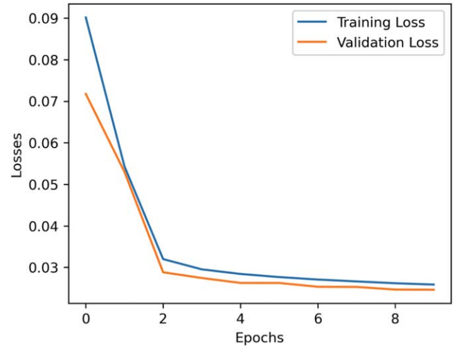
Figure 4. Training loss and validation loss during the 10 training epochs.
