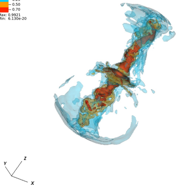
Fig. 1 Rendering of the 3D structure of the relativistic flows inside the nebula. The highest speeds ( v > 0.7c ) are achieved along the surface of the termination shock and, above all, in the polar jets produced by magnetic hoop stresses
