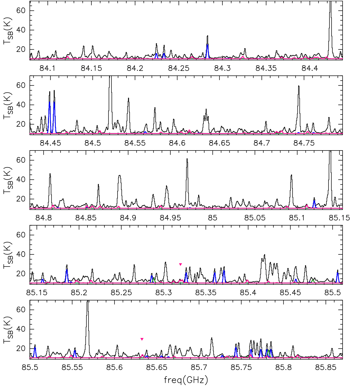
Fig. D.1. Total spectra of the GUAPOS project in black. In blue, we show the synthetic spectrum of the best fit of methyl formate (MF); in green the synthetic spectrum of the best fit of glycolaldehyde (GA); in pink the synthetic spectrum of the best fit of acetic acid (AA). The colored triangles indicate the transitions used to constrain the fitting procedure of the 3 different molecules. Closer views of those transitions are given in Figs. 5–7.
