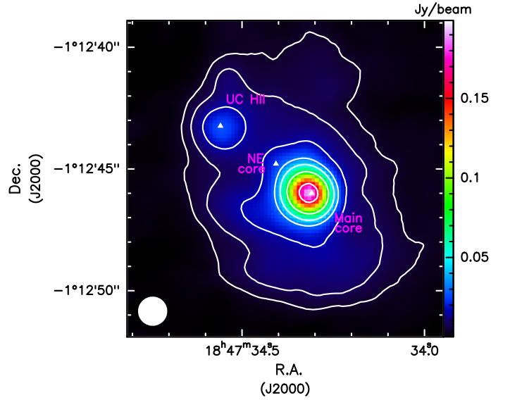
Fig. 2. Continuum map of the HMC G31.41+0.31 and the nearby UC HII region. Contour levels are at 5, 10, 20, 40, 60, 100, and 200 times the value of rms = 0.8 mJy beam -1 . The three white triangles indicate the coordinates of the Main Core and NE core by Beltrán et al. (2018), and of the UC HII region by Cesaroni et al. (1998). The beam is shown in white in the lower left corner.
