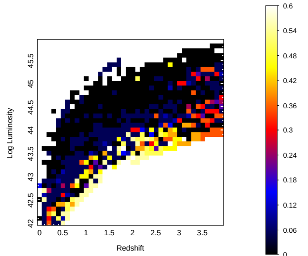
Fig. 5. Medians of the absorption correction U for the objects in the XMM-LSS, XMM-CDFS, and XMM-COSMOS surveys, over a grid of redshift and observed luminosity. Probability distributions for photometric redshifts have been included. The corrections are mostly significant for objects in the faint tail of the luminosity function (i.e. L \lesssim 43 – 44.5 , depending on z ), or for z \gtrsim 3 . The correction U (Sect. 3) is logarithmic, hence U = 0.5 corresponds to the luminosity being corrected by a factor of 2. The colour scale goes from black (median correction is 0) to bright yellow (median correction is 0.6). White areas are not populated.
