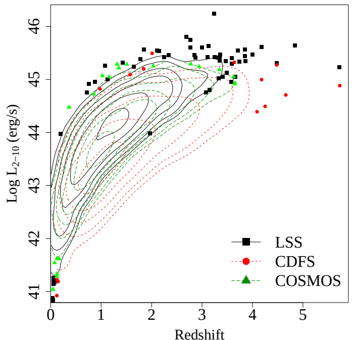
Fig. 2. Luminosity-redshift diagram for the XMM-LSS, XMM-CDFS, and XMM-COSMOS surveys. The contours are logarithmically scaled and show the fraction of objects with z and L inside the contour (levels at 97%, 94.8%, 90%, 83%, 70%, and 48% from outermost to innermost). The data points show the objects outside the lowest contour. At z > 0.5 , the XMM-CDFS systematically probes AGN that are fainter by up to one order of magnitude. Observed luminosities, corrected only for Galactic absorption, are shown.
