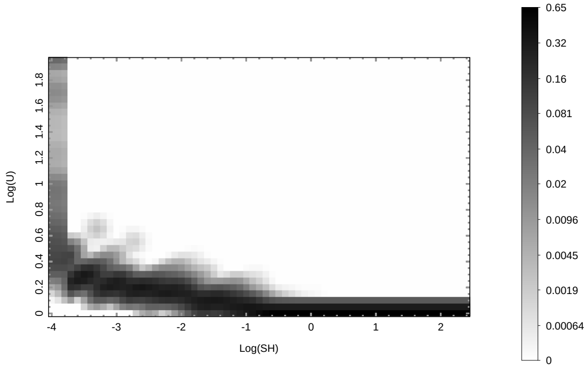
Fig. 4. Probability distribution of the unabsorbed/absorbed flux ratio in the 2–10 keV, as a function of the measured 0.5–2/2–10 keV flux ratio, for the Burlon sample, at redshift zero. The x-axis shows \text{Log}(SH) , therefore hard sources are on the left and soft sources are on the right. The y-axis shows \text{Log}(U) , therefore no correction is at the bottom and large corrections are at the top. The colour scale goes from white (low probability) to black (high probability).
