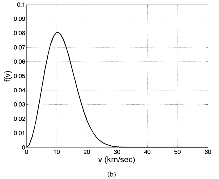
Fig. 6. Panel a: Micrometeoritic flux on Mars in the radius range between 5–100 \mu\text{m} of impacting particles. Panel b: Velocity distribution function of particles impacting Mars.
