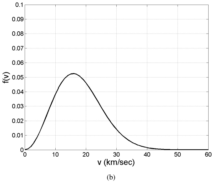
Fig. 5. Panel a: Micrometeoritic flux on Venus in the radius range between 5–100 \mu\text{m} of impacting particles. Panel b: Velocity distribution function of particles impacting Venus.
