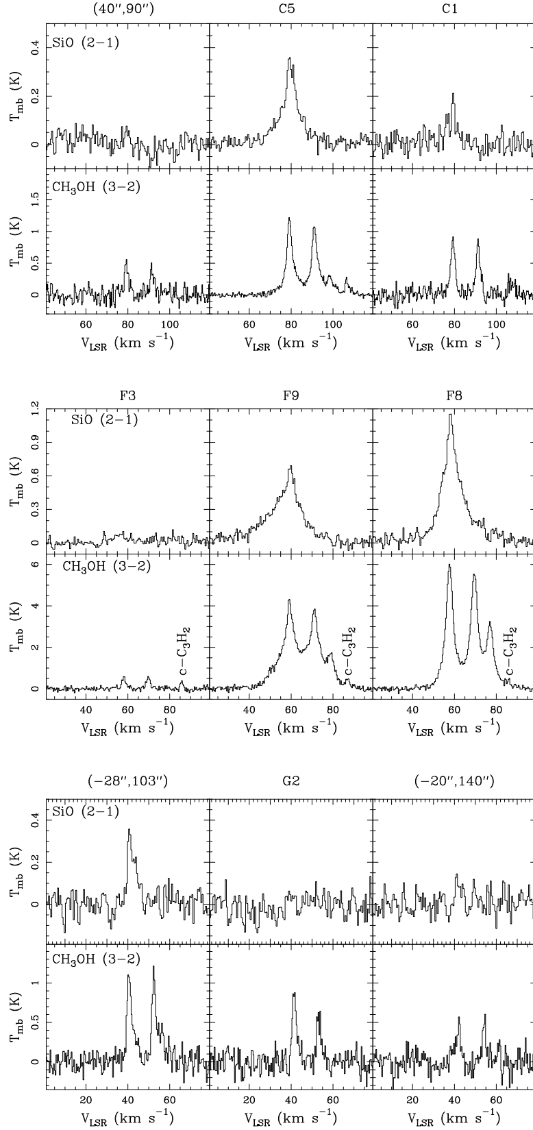
Figure 7. SiO and CH 3 OH spectra extracted toward three positions in cloud C (top panel), F (middle panel) and G (bottom panel). The corresponding position is indicated for every spectrum.
