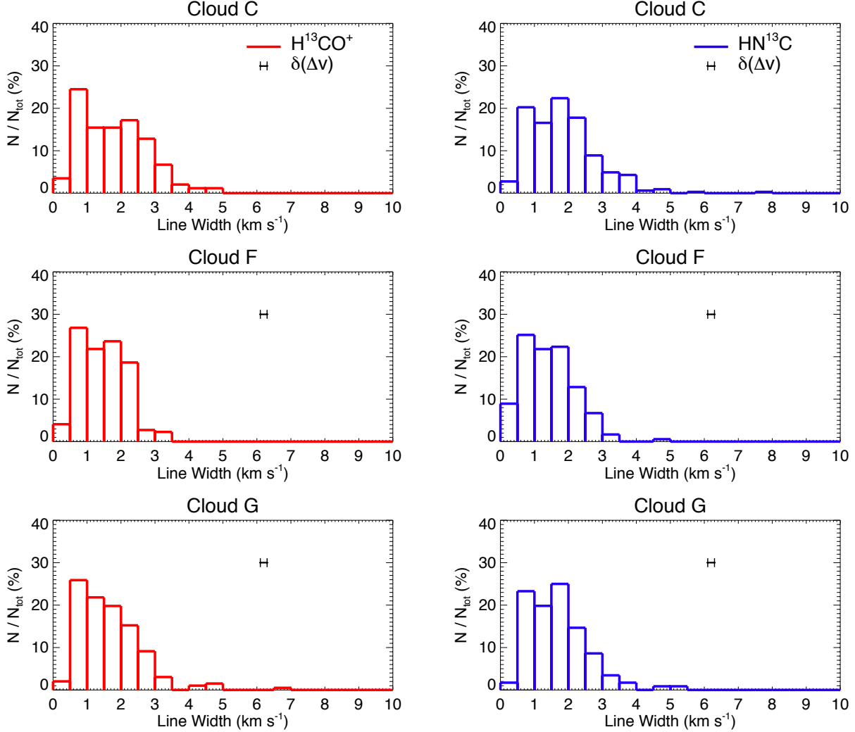
Figure 5. Line width distributions of the \text{H}^{13}\text{CO}^+ (left panels in red) and \text{HN}^{13}\text{C} (right panels in blue) emission measured for clouds C (top panels), F (middle panels) and G (bottom panels). The histograms show the percentage of emission lines having linewidths falling within each bin. Bin sizes are 0.5 \text{ km s}^{-1} for the three clouds, corresponding to 1/3 of the mean intensity-weighted linewidth. In each panel the mean uncertainty in the linewidth of the single fittings is indicated.
