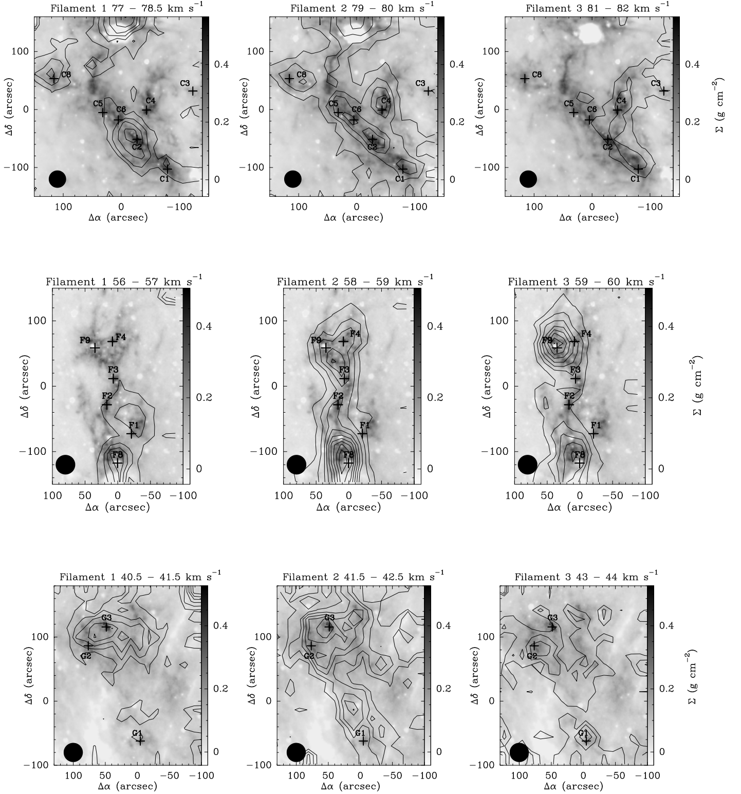
Figure 4. Integrated intensity maps of the \text{HN}^{13}\text{C} emission in clouds C (top panels), F (middle panels) and G (bottom panels) for the identified velocity sub-structures. The emission levels (black contours) are superimposed on the \text{H}_2 mass surface density map of Kainulainen & Tan (2013). The integrated velocity ranges are indicated in every panel and the emission levels go from 3\sigma by 3\sigma , where \sigma = 0.04 \text{ K km s}^{-1} for cloud C, \sigma = 0.04 \text{ K km s}^{-1} for cloud F and \sigma = 0.02 \text{ K km s}^{-1} for cloud G. The beam sizes are shown as black circles in all panels.
