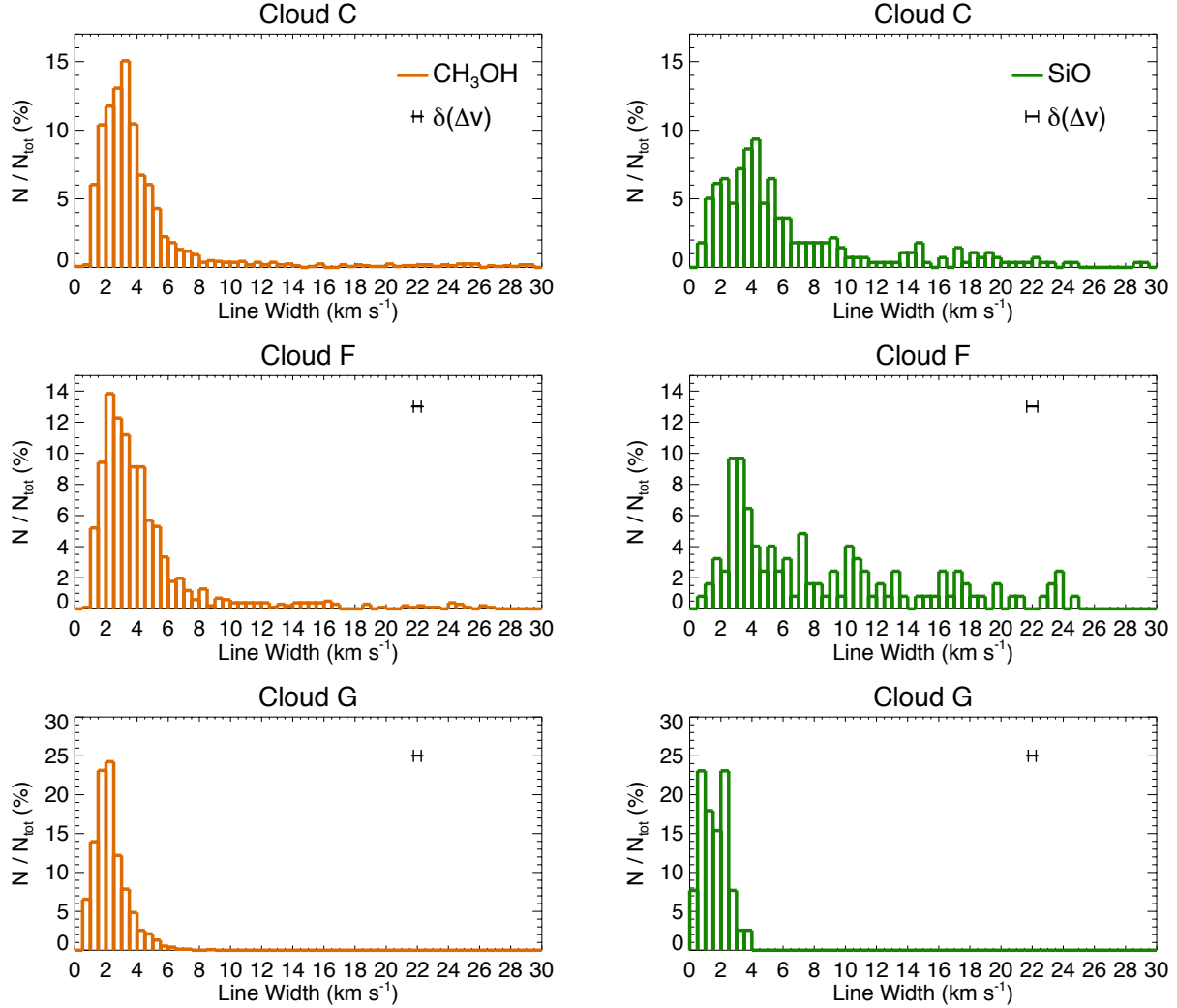
Figure 8. Line width distributions of the CH 3 OH (in orange) and SiO (in green) emissions obtained for clouds C (top panels), F (middle panels) and G (bottom panels). The histograms show the percentage of emission lines having line widths falling within each bin. Bin size for the CH 3 OH and SiO distributions are 0.5 km s -1 corresponding to 1/3 of the mean intensity-weighted linewidth obtained for the dense gas tracers. In each panel the mean uncertainty in the linewidths from the single fittings is indicated.
