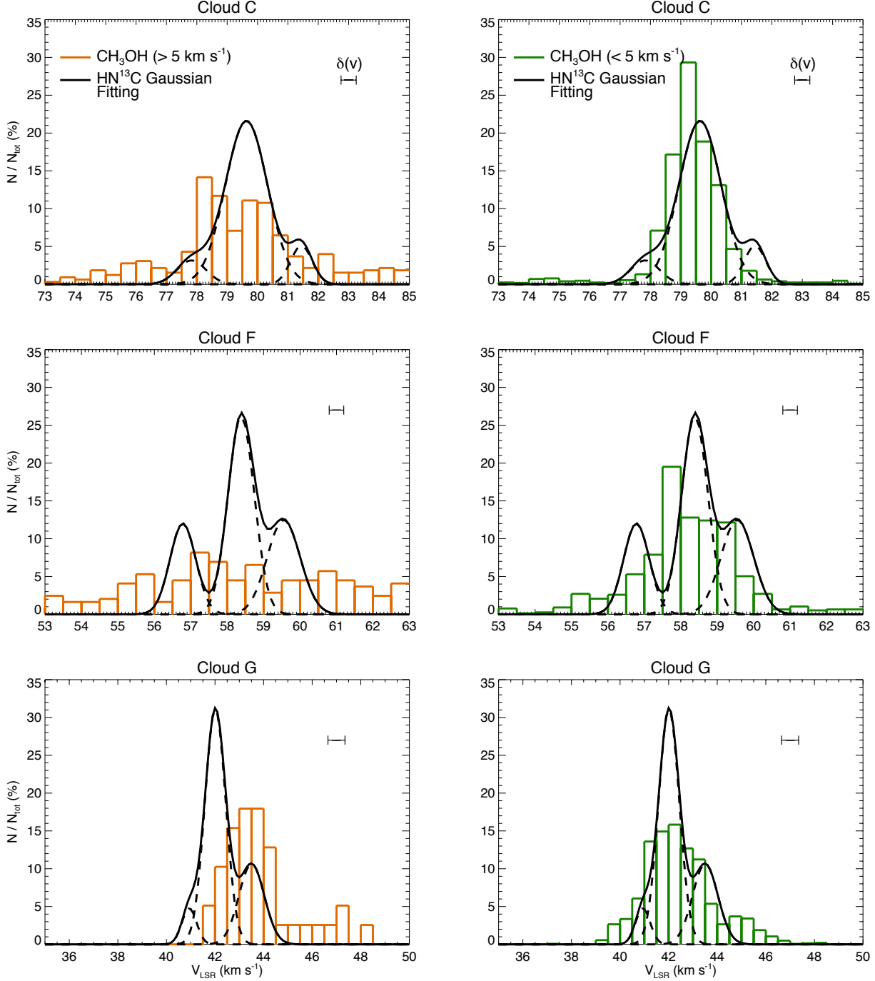
Figure 10. Velocity distribution of the CH 3 OH broad (linewidths > 5 \text{ km s}^{-1} , orange in left panels) and narrow (linewidths < 5 \text{ km s}^{-1} , green in right panels) emission obtained for clouds C (top panels), F (middle panels) and G (bottom panels). The histograms show the percentage of emission lines having radial velocities falling within each bin, with bin sizes 0.5 \text{ km s}^{-1} for the three clouds, corresponding to 1/3 of the mean intensity-weighted linewidth obtained for the dense gas tracers. The contribution from all CH 3 OH transitions detected in each cloud has been considered. In each panel, the mean uncertainty for the central velocities of the single fittings is indicated. Black curves correspond to the gaussian fitting obtained for HN 13 C in Section 4.1.1 (see also Figure 3).
