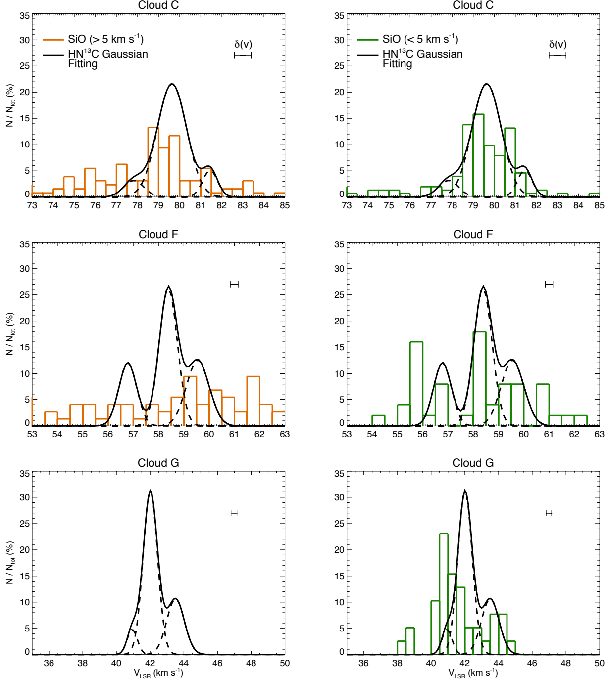
Figure 9. Velocity distribution of the SiO broad (with linewidths > 5 \text{ km s}^{-1} , orange in left panels) and narrow (with linewidths < 5 \text{ km s}^{-1} , green in right panels) emission obtained for cloud C (top panels), F (middle panels) and G (bottom panels). The histograms show the percentage of emission lines having radial velocities falling within each bin, where the bin size is 0.5 \text{ km s}^{-1} for the three clouds, corresponding to 1/3 of the mean intensity-weighted linewidth obtained for the dense gas tracers. In each panel, the mean uncertainty for the central velocities of the single fittings is indicated. Black curves correspond to the gaussian fitting obtained for \text{HN}^{13}\text{C} in Section 4.1.1 (see also Figure 3).
