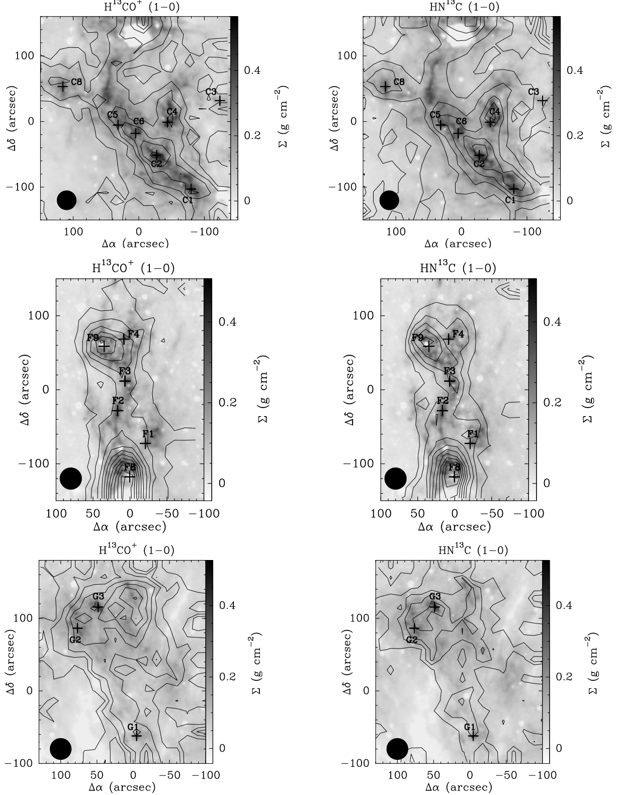
Figure 1. Integrated intensity maps of the \text{H}^{13}\text{CO}^+(1-0) (left) and \text{HN}^{13}\text{C}(1-0) (right) lines toward cloud C (top panels), F (middle panels) and G (bottom panels). Emission levels (black contours), from 3\sigma by 3\sigma , are superimposed on the \text{H}_2 mass surface density maps (gray scale) obtained by Kainulainen & Tan (2013). Cloud C : The integration range is 76 - 83 \text{ km s}^{-1} and \sigma = 0.10 \text{ K km s}^{-1} for both molecules. Cloud F : Integration range is 51 - 64 \text{ km s}^{-1} for both tracers and \sigma = 0.11 and 0.15 \text{ K km s}^{-1} for \text{H}^{13}\text{CO}^+ and \text{HN}^{13}\text{C} respectively. Cloud G : Integration range is 39 - 45 \text{ km s}^{-1} ; \sigma = 0.09 and 0.06 \text{ K km s}^{-1} for \text{H}^{13}\text{CO}^+ and \text{HN}^{13}\text{C} , respectively. The core positions (black crosses; Butler & Tan 2009, 2012) and the beam sizes (black circles) are shown in all panels.
