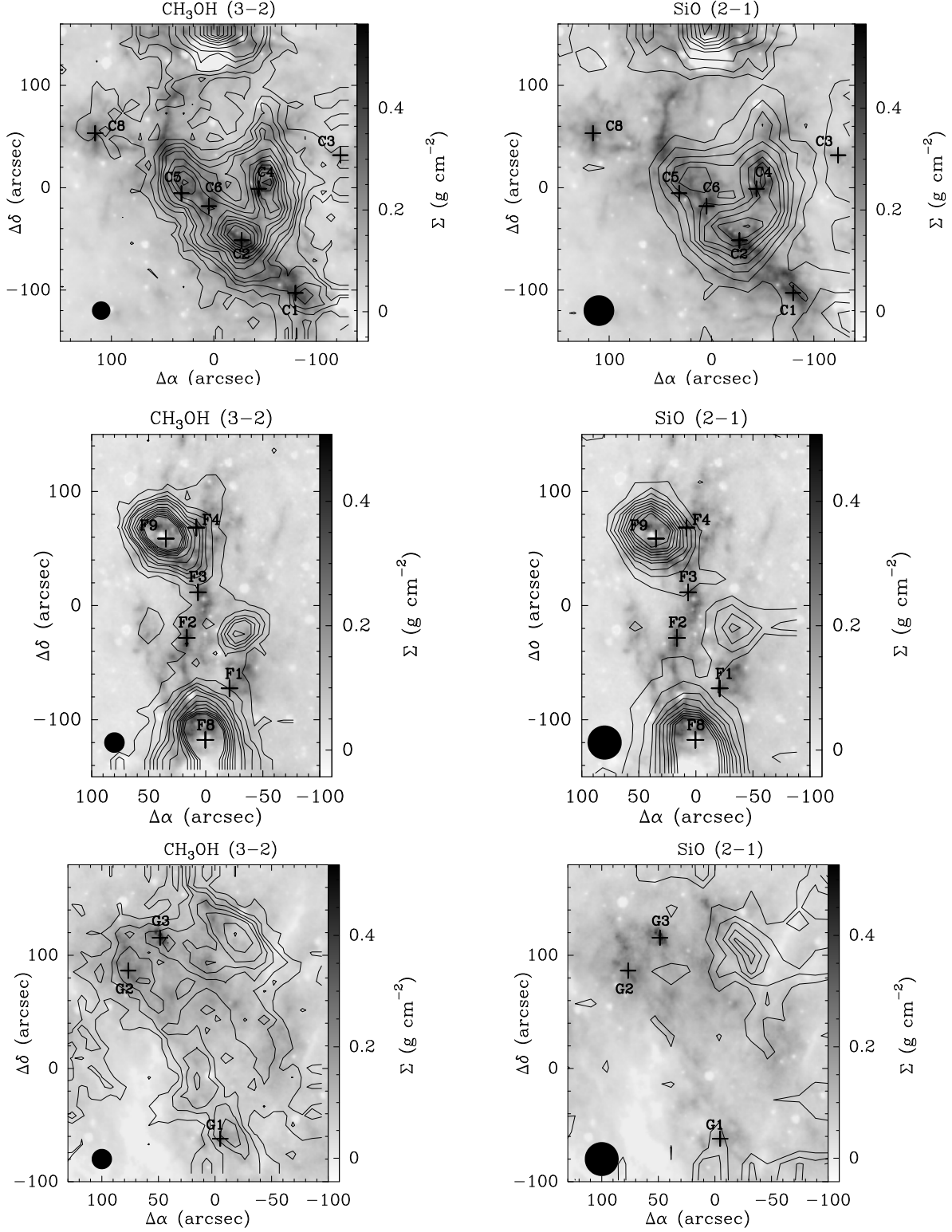
Figure 6. Integrated intensity maps of the CH 3 OH(3-2) (left) and SiO (2-1) (right) lines toward cloud C (top panels), F (middle panels) and G (bottom panels). Emission levels (black contours) are 3\sigma , 6\sigma , 9\sigma , 12\sigma , 15\sigma , 21\sigma , 27\sigma , 33\sigma , 39\sigma , 45\sigma , 51\sigma and 57\sigma for CH 3 OH; 3\sigma , 6\sigma , 9\sigma , 12\sigma , 15\sigma , 18\sigma , 21\sigma , 24\sigma , 27\sigma and 30\sigma for SiO. The contours are superimposed on the H 2 mass surface density maps (gray scale) obtained by Kainulainen & Tan (2013). Cloud C : The integration ranges are 65 - 90 km s -1 for SiO and 75 - 85 km s -1 for CH 3 OH and \sigma = 0.20 K km s -1 for both molecules. Cloud F : The integration ranges are 40 - 80 km s -1 for SiO and 52 - 64 km s -1 for CH 3 OH. \sigma = 0.24 and 0.25 K km s -1 for SiO and CH 3 OH respectively. Cloud G : Integration ranges are 35 - 50 km s -1 for SiO and 38 - 50 km s -1 for CH 3 OH; \sigma = 0.10 and 0.20 K km s -1 for SiO and CH 3 OH, respectively. The core positions (black crosses; Butler & Tan 2009, 2012) and the beam sizes (black circles) are shown in all panels.
