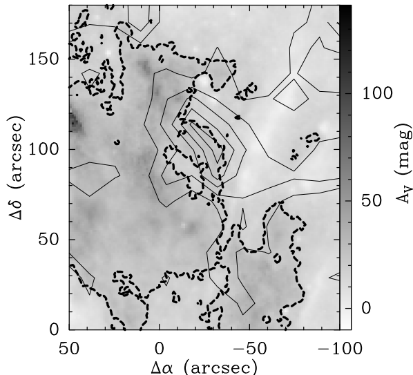
Figure 11. Integrated intensity map of the SiO line emission observed toward cloud G (solid contours) and superimposed on the A_v visual extinction map (gray scale) derived by Kainulainen & Tan (2013). The velocity range for the SiO integrated intensity map is 35 - 50 km s -1 and the contour levels are 3 \sigma , 6 \sigma , 9 \sigma , 12 \sigma and 15 \sigma ( \sigma = 0.1 K km s -1 ). Dashed contour corresponds to a visual extinction of A_v = 20 mag.
