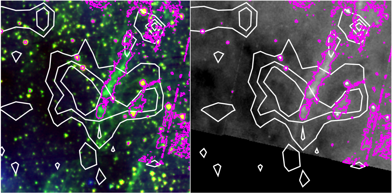
Figure 12. Comparison of the SiO emission (white contours) with emissions at 3.6 \mu\text{m} , 4.5 \mu\text{m} , 8 \mu\text{m} and 24 \mu\text{m} , toward cloud G as obtained with the Spitzer Telescope . Left panel: Spitzer 3-color image with 3.6 \mu\text{m} emission displayed in red, 4.5 \mu\text{m} emission in green and 24 \mu\text{m} emission in blue. Right panel: 8 \mu\text{m} emission toward cloud G displayed in gray scale. In both panels the SiO emission levels (white contours) correspond to 3\sigma , 6\sigma and 9\sigma , with \sigma = 0.1 \text{ K km s}^{-1} . The 4.5 \mu\text{m} nebula is highlighted by the magenta contour corresponding to the 12\sigma level at 4.5 \mu\text{m} and 100\sigma level at 8 \mu\text{m} .
