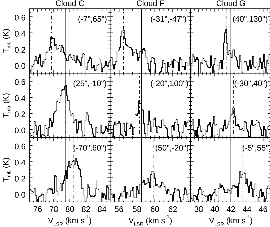
Figure 2. \text{HN}^{13}\text{C} spectra for clouds C (left panel), F (middle panel) and G (right panel) extracted toward several positions and highlighting the presence of multiple velocity components. The vertical solid lines correspond to the central velocity of the clouds while the vertical dot-dashed lines indicate the central velocity of the spectrum peaks. The same result has been found for the \text{H}^{13}\text{CO}^+ emission in all the three clouds and are not shown for simplicity.
