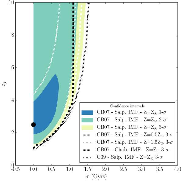
Figure 4. Star formation history confidence intervals contours. The 1-, 2- and 3- \sigma contours (respectively shown in blue, green and yellow) representing the quality of the fit between observed BCGs i - z colour evolution and a CB07 model with Z=Z_{\odot} and Salpeter IMF. The other dashed lines represent various 3- \sigma contours obtained for different IMF or metallicity choices. The fit with the lowest \chi^2 value is represented by the black dot and corresponds to CB07 model with a single-stellar population, solar metallicity and Salpeter IMF.
