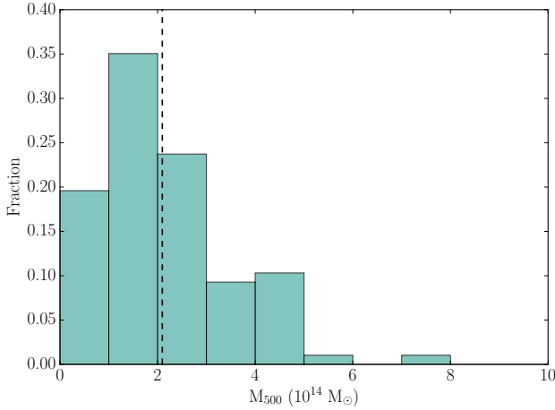
Figure 1. Normalized mass distribution obtained from X-ray scaling relations for XXL-100-GC. The dashed vertical line indicate the average XXL-100-GC cluster mass of just over 2 \times 10^{14} \text{ M}_{\odot} .
