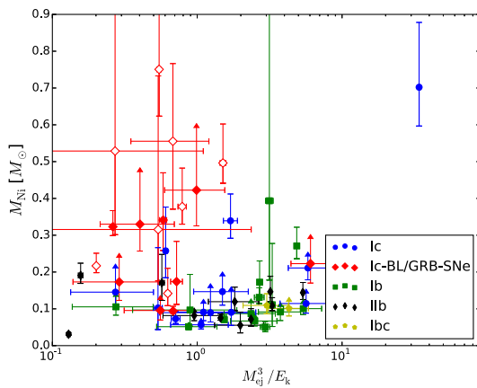
Figure 21. Nickel mass as a function of M_{ej}^3/E_k . Open symbols represent GRB-SNe.
