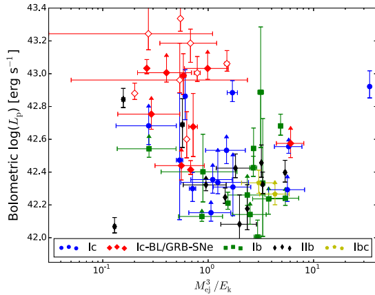
Figure 20. Peak bolometric luminosity as a function of M_{ej}^3/E_k . Open symbols represent GRB-SNe.
