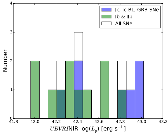
Figure 10. The luminosity function derived from the peak luminosity of the 18 UBVR/NIR LCs in the sample. Median host-galaxy extinction is assumed in three cases for statistical purposes. Colours are as described in Fig. 9.
