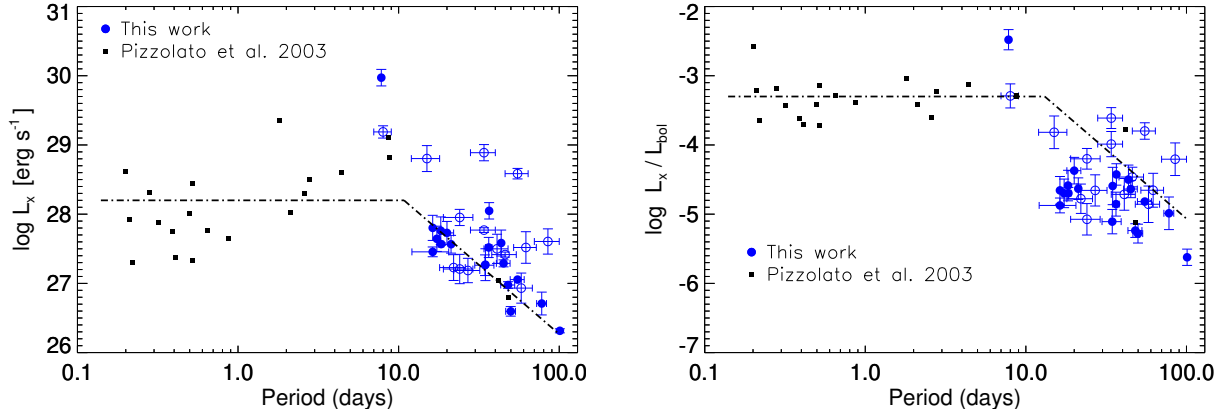
Fig. 4. L_x (left) and L_x/L_{bol} (right) vs. rotation period. The black squares correspond to the stellar sample from Pizzolato et al. (2003) in the mass range 0.22 < M/M_\odot < 0.60 . The large blue dots correspond to the M dwarfs with periods measured from time series and used in the analysis. The open blue circles show the derived period from an activity–rotation relation (excluded from the analysis). The black dot-dashed line represents the broken power law obtained by the fitting procedure from Pizzolato et al. (2003) with P_{rot} values estimated from v \sin i in saturated regime.
