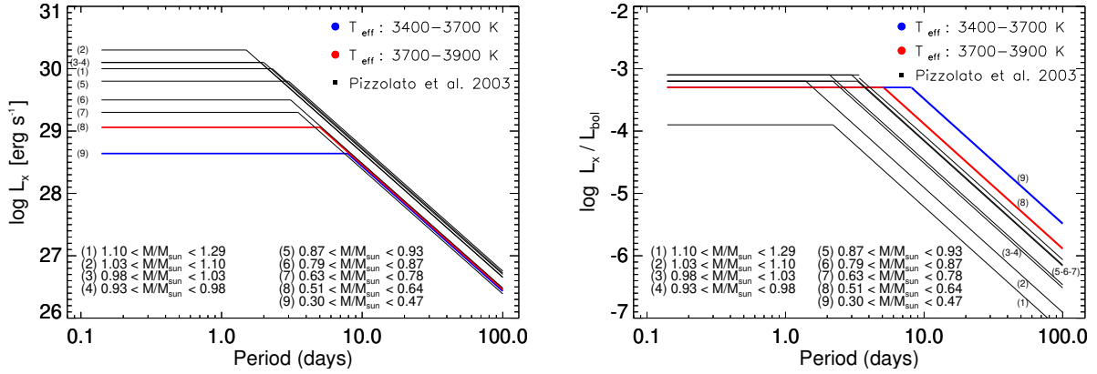
Fig. 6. All the best-fit relations between X-ray emission and rotational period for all the mass ranges (F to K stars) considered in Pizzolato et al. (2003) are presented as black lines. The blue and red solid line represents our best fit for the 3400–3700 and 3700–3900 K T_{\text{eff}} range, respectively.
