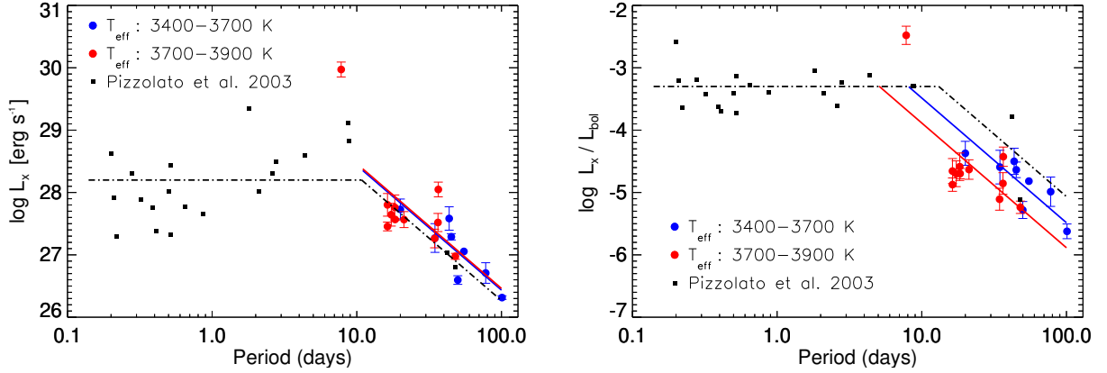
Fig. 5. L_x (left) and L_x/L_{bol} (right) vs. rotation period for stars with direct rotation period determination. The black squares correspond to the stellar sample from Pizzolato et al. (2003) in the mass range 0.22 < M/M_\odot < 0.60 . The blue and red dots correspond to the M dwarfs from this work in the two different ranges of T_{eff} indicated in the legend. The black dot-dashed line represents the broken power law obtained by the fitting procedure from Pizzolato et al. (2003). The blue and red solid line represents our best fit for the 3400–3700 and 3700–3900 K T_{eff} range, respectively.
