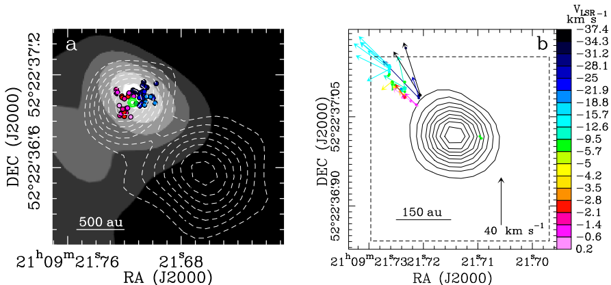
Figure 1. Previous NOEMA, JVLBA and VLBA observations towards IRAS 21078+5211. (a) The gray-scale (from 10 to 35 mJy beam -1 ) map reproduces the NOEMA 1.37 mm continuum emission (Moscadelli et al. 2021). The colored dots represent the channel emission peaks of the \text{CH}_3\text{CN} J_K = 12_K - 11_K ( K = 3-6 ) and \text{HC}_3\text{N} J = 24-23 lines, with colors denoting the channel V_{\text{LSR}} : blue for [-13.6, -10] and red [-2.5, 0.5] km s -1 . The green (70%, 80%, and 90% of 0.50 mJy beam -1 ) and white (from 30% to 90%, in steps of 10% of 0.096 mJy beam -1 ) contours show the JVLBA A-Array continuum at 1.3 cm and 5 cm, respectively. (b) Colored dots and arrows give absolute positions and proper motions of the 22 GHz water masers determined with multi-epoch (2010–2011) VLBA observations (Moscadelli et al. 2016), with colors denoting the maser V_{\text{LSR}} . The black contours (from 10% to 90%, in steps of 10% of 0.50 mJy beam -1 ) indicate the JVLBA A-Array continuum at 1.3 cm. The dashed rectangle delimits the field of view plotted in Fig. 2a.
