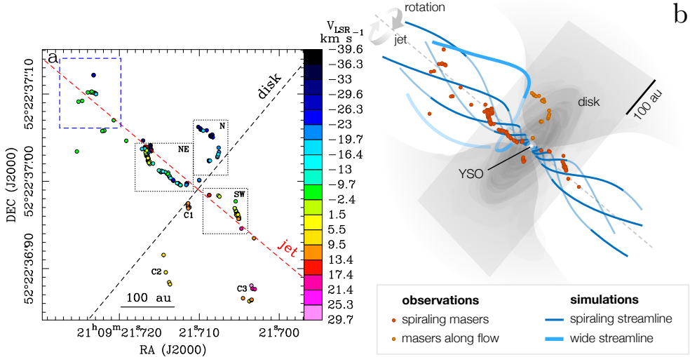
Figure 2. Global VLBI observations of the 22 GHz water masers and 3D view of the proposed kinematical interpretation (Moscadelli et al. 2022). (a) Colored dots give absolute positions of the 22 GHz water masers, with colors denoting the maser V_{\text{LSR}} . The black dotted rectangles encompass the three regions, to the N, NE and SW, where maser emission concentrate. The blue dashed rectangle delimits the area of maser emission in the previous VLBA observations. The red and black dashed lines mark the sky-projected jet and disk axis, respectively. (b) Observed maser positions (red and orange dots) overlaid on top of streamlines (blue curves) computed from resistive-radiative-gravito-MHD simulations of a jet around a forming massive star. The streamlines close to the rotation axis show significant spiraling motion, in agreement with the kinematic signature of the masers observed in the NE and SW regions. The wide streamline from the simulation illustrates the outflowing trajectory of material from the outer disk, similar to the observed masers in the N region. For context, the protostar, the disk and the outflow cavity have been sketched in gray, based on the density structure obtained in the simulations.
