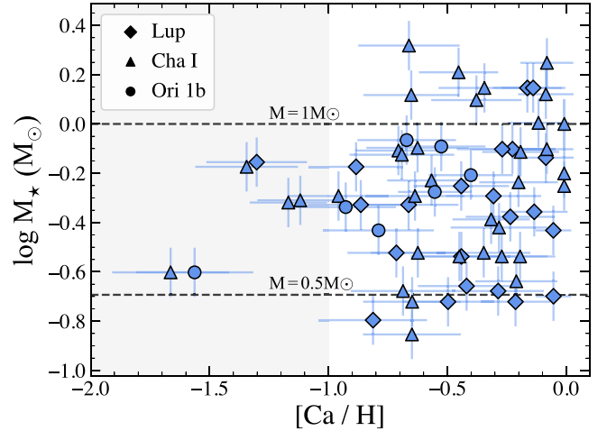
Figure 3. [\text{Ca}/\text{H}] vs. M_* . The gray region highlights the [\text{Ca}/\text{H}] \leq -1 region, the minimum abundance we are able to detect for M_* > 1 . No relationship between the stellar mass and Ca abundance is found.
