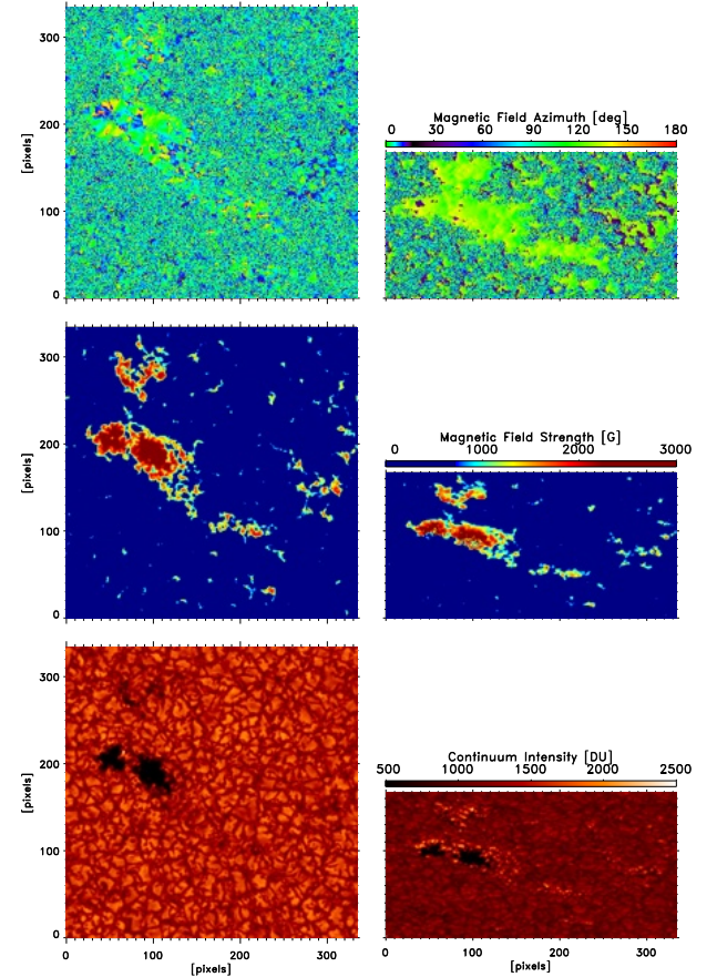
Fig. 5. MHD simulation of a realistic active region as seen at disk center (left panels) and at a heliocentric angle of \theta = 60^\circ (right panels). The synthesized spectra have been degraded using the instrumental parameters of the PHI-HRT telescope at a solar distance of 0.28 AU and subsequently inverted.
