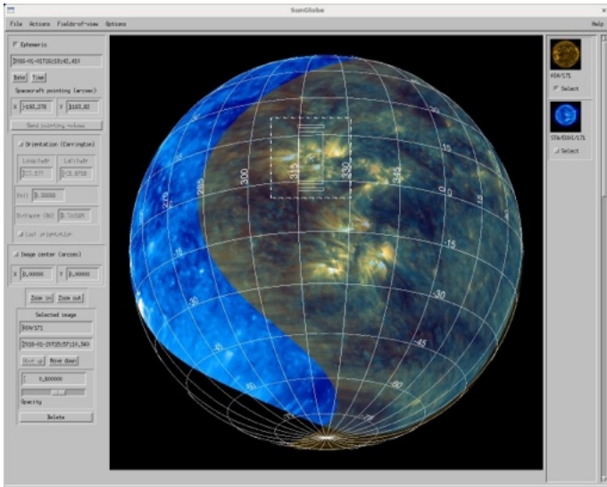
Fig. 19. SunGlobe program, showing the fields-of-view of SPICE, EUI, and PHI for a selected S/C pointing.
