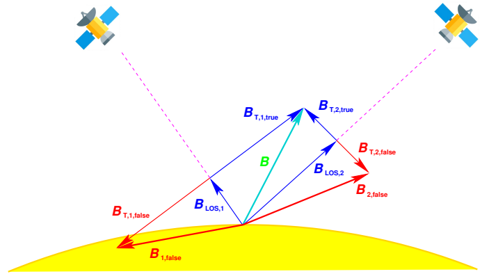
Fig. 4. Sketch of the ambiguity arising by deriving the magnetic field vector using the Zeeman effect. Observations from a single vantage point allows for two different solutions \mathbf{B} or \mathbf{B}_{1,false} . Stereoscopic observations make possible the selection of the correct solution between \mathbf{B} , \mathbf{B}_{1,false} and \mathbf{B}_{2,false} .
