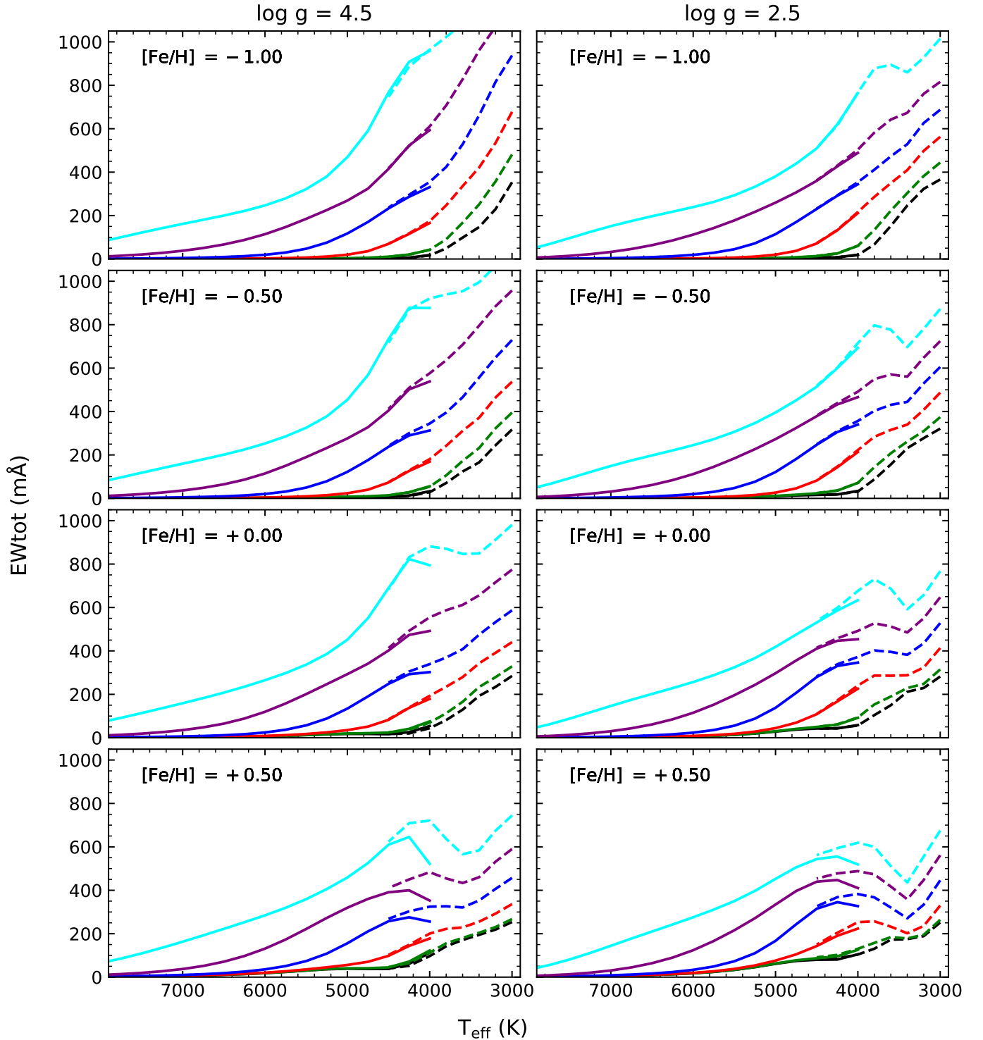
Fig. 5. Comparison of the measured total EW(Li + Fe) vs. T_{\text{eff}} for FGK (solid lines) and M-type stars with v \sin i = 0 (dashed lines), for \log g = 4.5 (left panels) and 2.5 (right panels), and different metallicities. The COGs are plotted for A(\text{Li}) = -1.0 (black), 0.0 (green), +1.0 (red), +2.0 (blue), +3.0 (purple), and +4.0 (cyan).
