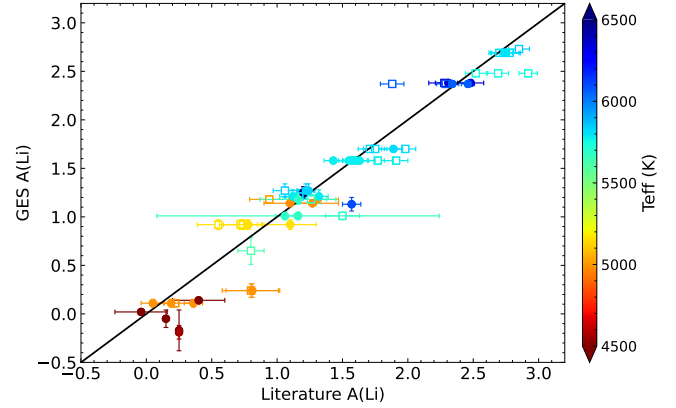
Fig. 13. Comparison of the average GES abundances for benchmark stars with those from the AMBRE project (open squares, Guiglion et al. 2016) and from other literature studies (filled circles, see text). Only stars with detections in GES and in the literature studies are plotted. Data are colour-coded by the GES temperature. Points aligned on the same horizontal line refer to multiple measures of the same star.
