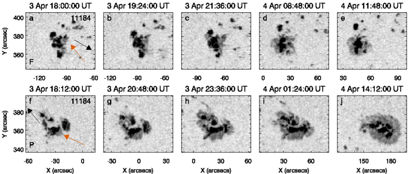
Figure 8. Same in Figure 4, for AR 11184.
