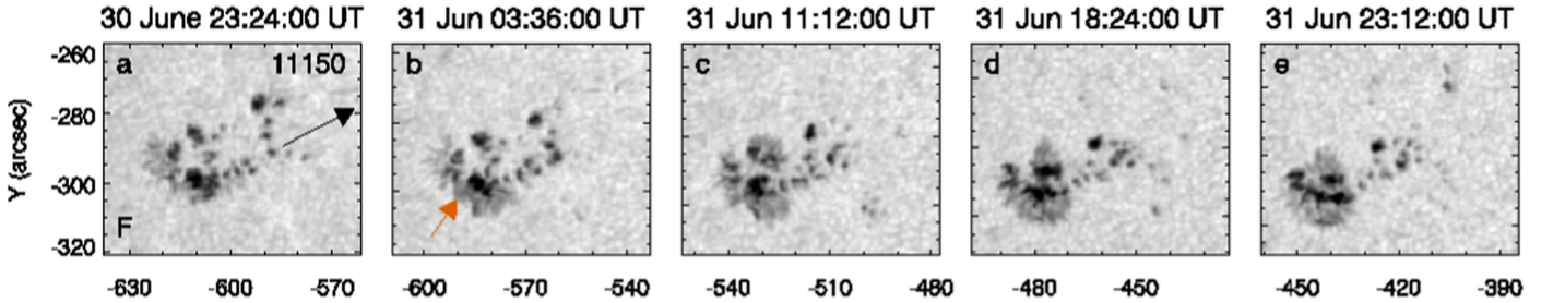
Figure 7. Same as Figure 4 for the following polarity of AR 11150
