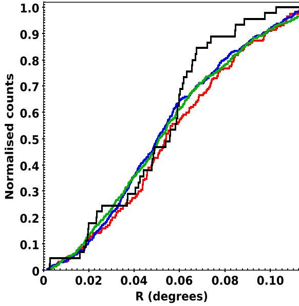
Figure 13. Cumulative radial distributions of selected samples of sources in the CMD of And XXI. Green line: cumulative distribution for the RGB stars; blue line: distribution of the red-HB stars; red line: distribution of the upper-HB sources; black line: distribution of the variable stars.
