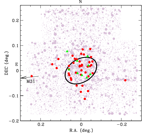
Figure 4. Spatial distribution of the variable stars detected in And XXI. Red filled circles mark the RR Lyrae stars and green filled triangles are the ACs. Symbol size for all other stars is proportional to the magnitude. An ellipse marks the area enclosed in the half-light radius defined by Martin et al. (2009). The arrow marks the direction toward the M31 center.
