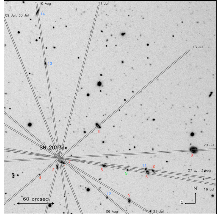
Fig. 8. Field of SN 2013dx with the slit positions used for FORS2 spectroscopy overimposed. Each slit position is identified by its observation date. Numbers mark the galaxies for which spectroscopic detection was secured. Red numbers refer to galaxies with redshift close to that of the SN 2013dx host galaxy ( z = 0.145 ). Blue numbers refer to galaxies not related to the SN. The green “S” marks a field star included in the slit on 16 July.
