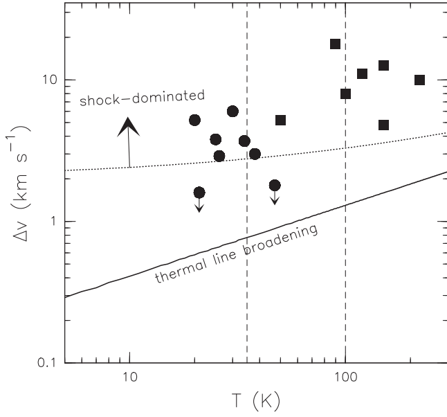
Figure 2. Line widths derived from the PN (2–1) line in this work (circles) and in Turner et al. (1990; squares) against the gas kinetic temperature. The vertical dashed lines indicate the desorption temperatures predicted by the theoretical model of Charnley & Millar (1994), i.e., 100 \pm 15 K, and the possible smaller one derived from Garrod & Herbst (2006) of \sim 35 K. The expected thermal line broadening, \Delta v_{\text{th}} , is indicated by a solid oblique line. Finally, the dotted line marks an arbitrary threshold of \Delta v_{\text{non-th}} \simeq 2 \text{ km s}^{-1} (where \Delta v_{\text{non-th}} represents the non-thermal component of the line), corresponding to about 10 times \Delta v_{\text{th}} for T \sim 5 K, in which the internal motions likely start to be affected by shock-induced turbulence. The two circles with arrows indicate 18517+0437 and 19410+2336, for which the line width was derived from a Gaussian fit; hence, it represents an upper limit to the intrinsic line width.
