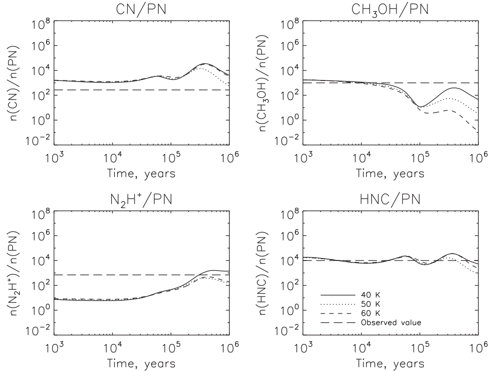
Figure 3. Volume density ratios as a function of time of the species indicated on top of each panel, calculated from the chemical models described in Section 4. Straight, dotted, and dashed curves represent a constant temperature of 40, 50, and 60 K, respectively. The long-dashed line in each frame indicates the observed average density ratios (see Section 4).
