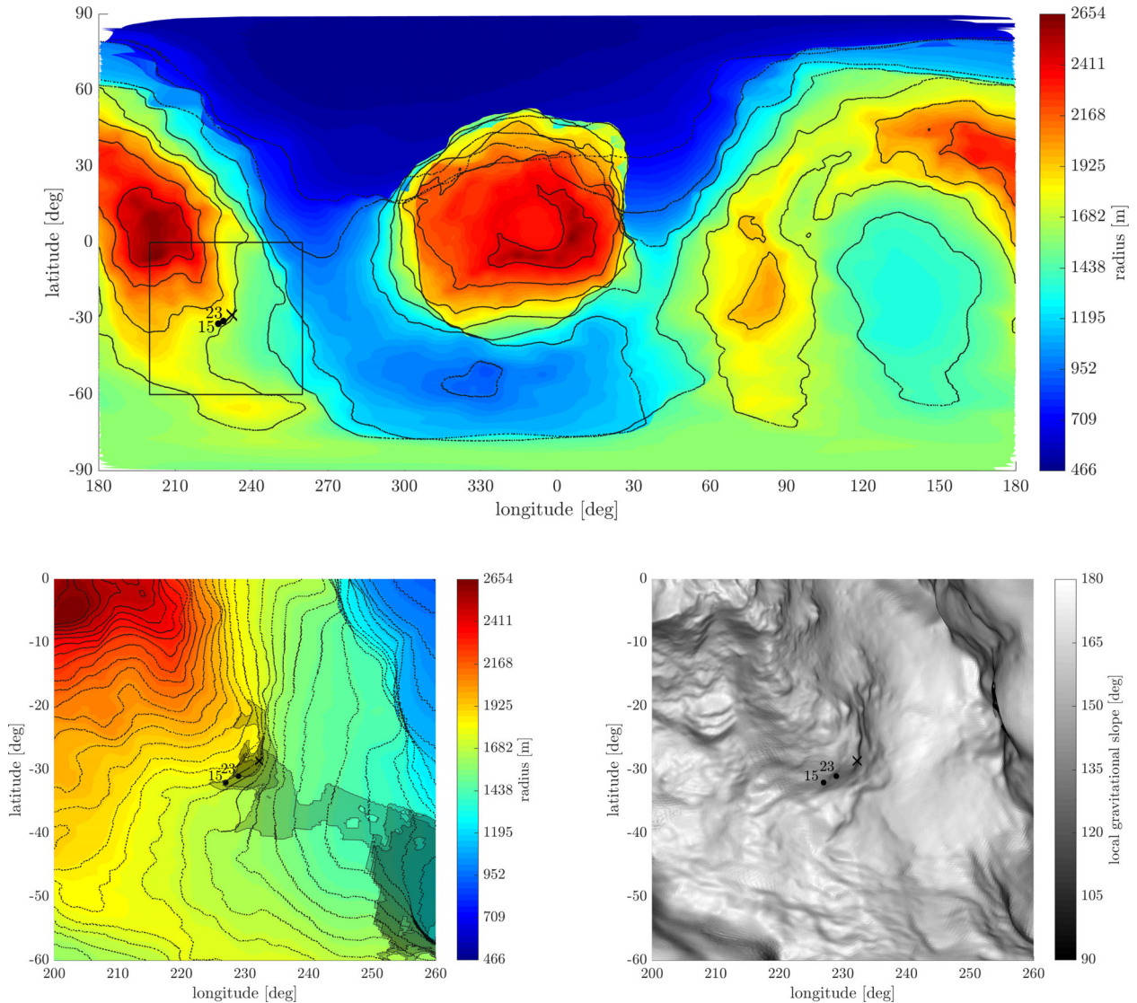
Figure 20. Terrain maps of 67P. Outburst positions are marked by X (2016 Feb 19 outburst) and by numbers (cf. Vincent et al. 2016b). Top: radius map showing the elevated head region in the centre and the body at the left (West) and right (East) fringes. Lower left: enlarged radius map showing the outburst position (x). The contour lines are separated by 50 m. Grey shading represent illuminated areas at 09:40 (dark grey), 09:50 (middle grey), and 10:00 (light grey). Lower right: topographic map in which the grey shading represents the local slope, accounting for gravity and centrifugal force (white=flat, black=vertical wall).
