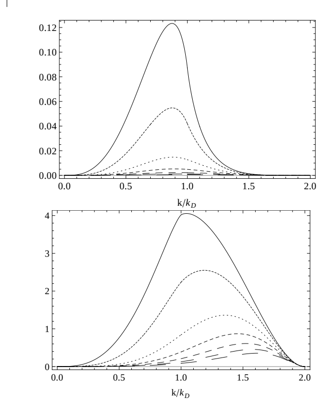
FIG. 6. Comparison of antisymmetric correlators in units of \langle B^2 \rangle \langle \mathcal{B}^2 \rangle / (4\pi)^4 , the different lines are for n_B = n_H = -3/2, -1, 0, 1, 2, 3, 4 ranging from the solid to the longest dashed. The vector one, k^3 X^{(V)}(k) , in the upper panel and the tensor one, k^3 X^{(T)}(k) , in the bottom panel.
