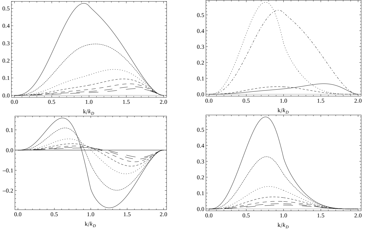
FIG. 1. Non-helical (helical) contribution to k^3 |\rho(k)|^2 in units of \langle B^2 \rangle^2 / (4\pi)^4 ( \langle \mathcal{B}^2 \rangle^2 / (4\pi)^4 ) versus k/k_D is plotted in the upper left (bottom left) panel. The total contribution is displayed in the bottom right panel for \langle B^2 \rangle^2 = \langle \mathcal{B}^2 \rangle^2 and n_B = n_H . The different lines are for n_B ( n_H ) = -3/2, -1, 0, 1, 2, 3, 4 ranging from the solid to the longest dashed. The panel in the upper right display the comparison between the non-helical case and the maximal helical case for n_{B,H} = 1 (solid vs dashed) and n_{B,H} = -3/2 (dot-dashed vs dotted).
