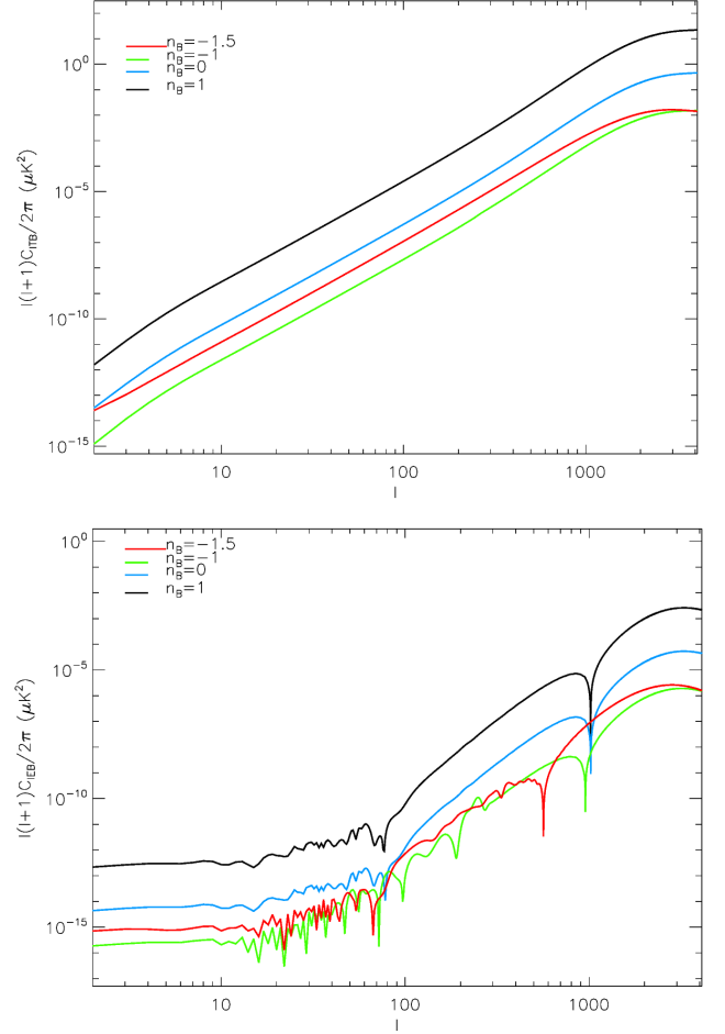
FIG. 9. On the top panel we show the parity-odd vector power spectrum TB and in the bottom panel the parity-odd correlator EB , with a magnetic field \sqrt{\langle B_\lambda^2 \rangle} = 3.5 \text{ nG} .
