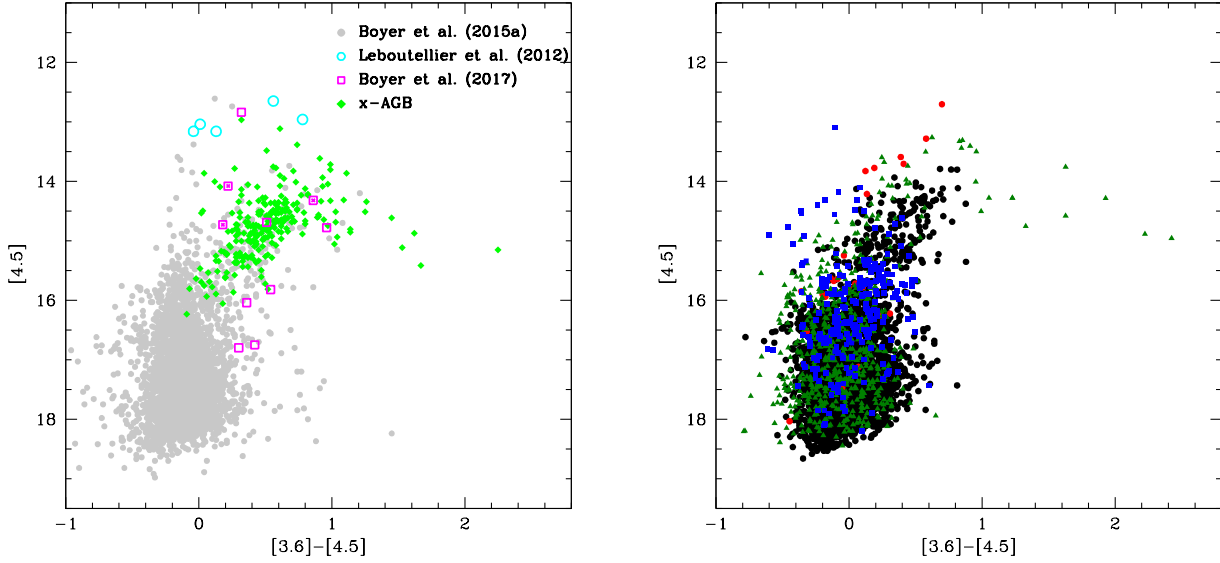
Figure 7. Left: The distribution on the colour-magnitude ( [3.6] - [4.5] , [4.5] ) plane of the IC10 stars from Boyer et al. (2015a), indicated with grey points. Cyan circles indicate the bright, O-rich stars by Leboutellier et al. (2012), whereas the obscured stars by Boyer et al. (2017), classified as O-rich, are indicated with magenta squares (crosses inside the square mean variable sources). The x-AGB stars by Boyer et al. (2015b) are represented with light green diamonds. Right: The results from synthetic modelling, with the same symbols used in Fig. 4 and 5.
