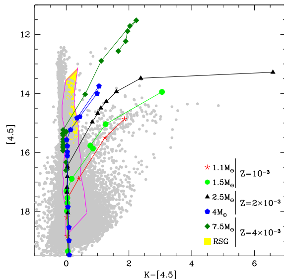
Figure 1. The evolutionary tracks of stars of various mass and metallicity are overlaid to the observations in the colour-magnitude (K - [4.5], [4.5]) plane. The yellow region, delimited by a magenta track, points the locus of the plane populated by stars of mass in the range 6 - 20 M_{\odot} during the core helium-burning phase. See the text for the choices regarding the assumed reddening and distance of IC10.
