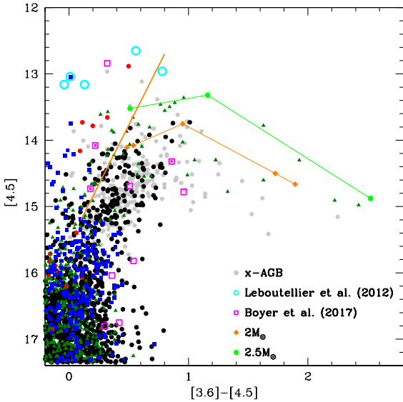
Figure 8. The distribution of IC10 x-AGB stars by Boyer et al. (2015b) (grey points), the stars from Leboutellier et al. (2012) (cyan circles) and Boyer et al. (2017) (magenta squares) on the colour-magnitude ( [3.6] - [4.5] , [4.5] ) plane. Results from synthetic modelling are also shown, with the same symbols of Fig. 4 and 5. The evolutionary tracks of stars of initial mass 2 M_{\odot} (orange) and 2.5 M_{\odot} (light green) are shown.
