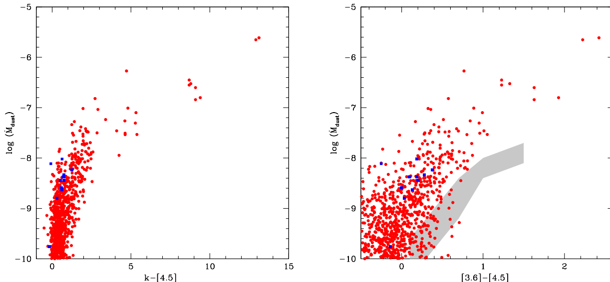
Figure 9. The dust mass loss rate of the stars in our synthetic population, as a function of the K - [4.5] (left panel) and [3.6] - [4.5] (right) colours. Red points indicate carbonaceous dust, whereas blue squares indicate silicate and alumina dust production. The grey, shaded region in the right panel indicate the relation for SMC AGB stars, given in Srinivasan et al. (2016).
