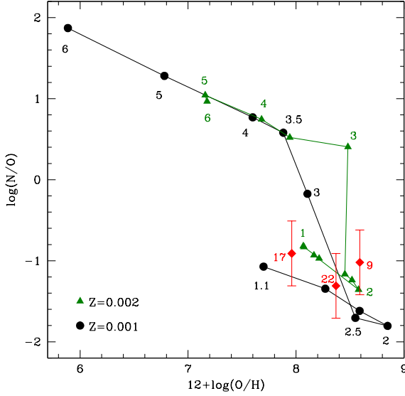
Figure 10. Red diamonds indicate the chemical composition of the 3 PNe in IC10 studied by Magrini & Goncalves (2009), for which both the O and N measurements are available. Black points and green triangles points the final chemistry of AGB models of mass in the range 1-6 M_{\odot} and metallicity, respectively, Z = 10^{-3} and Z = 2 \times 10^{-3} .
