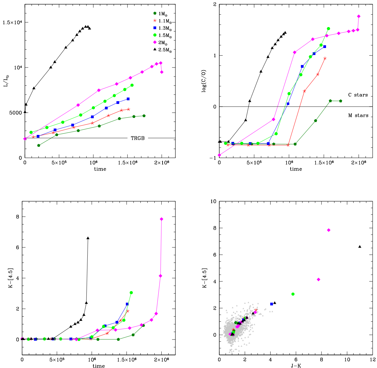
Figure 2. The evolution of the luminosity (top, left panel) and of the C/O ratio (top, right) of 1\text{--}2 M_{\odot} at Z = 10^{-3} and 2.5 M_{\odot} at Z \leq 2 \times 10^{-3} . The thin, horizontal lines mark the location of the TRGB and the boundary between M stars and carbon stars. The variation of the (K-[4.5]) colour is shown in the bottom, left panel. We also show the excursion of the tracks in the colour-colour ( J-K ) vs (K-[4.5]) plane, overimposed to the data of the IC10 evolved stellar population by Gerbrandt et al. (2015) and Boyer et al. (2015a). The adopted reddening is E(B - V) = 1.14 mag (see section 5.2)
