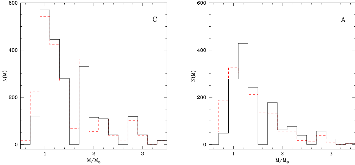
Figure 6. The progenitors mass distribution (black, solid lines) and the current mass (red, dashed) of the stars populating region C (left panel) and A (right) in Fig. 5.
