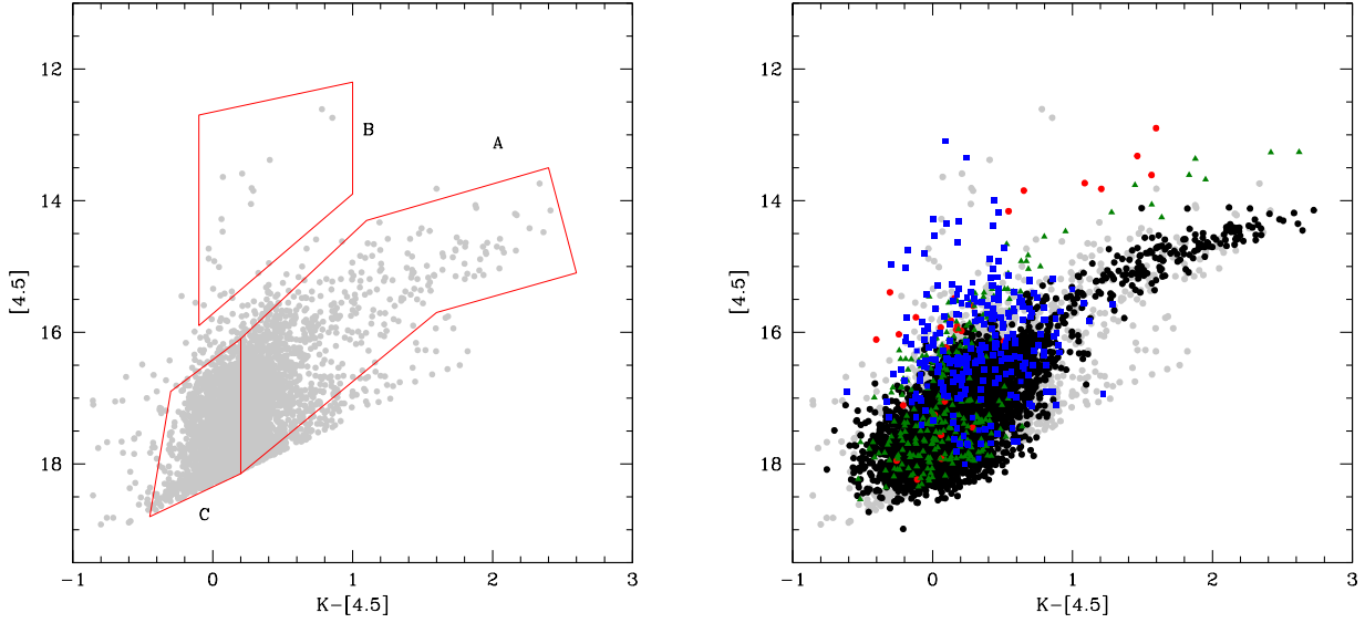
Figure 4. Left: The distribution of IC10 stars in the colour-magnitude ( K-[4.5] , [4.5] ) plane. Right: The results from population synthesis, obtained by adopting the recommended SFH by Weisz et al. (2014). The different colours indicate stars of metallicity Z = 10^{-3} (black points, initial masses below 2 M_{\odot} ), Z = 2 \times 10^{-3} (green triangles, descending from stars of mass 2 M_{\odot} < M < 4 M_{\odot} ), Z = 4 \times 10^{-3} (red points, initial mass above 4 M_{\odot} ), core helium-burning stars (blue squares, also assumed to have a metallicity Z = 4 \times 10^{-3} ). The observed sample is also shown as light-grey points in the right panel.
